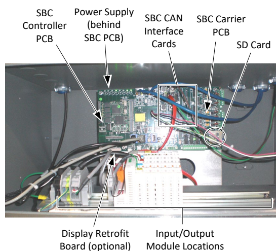
Fig. 8.4. Master Controller
