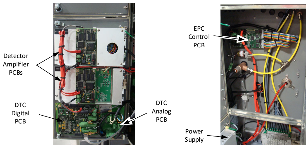
Fig. 6.5. Class C Oven Component Locations
