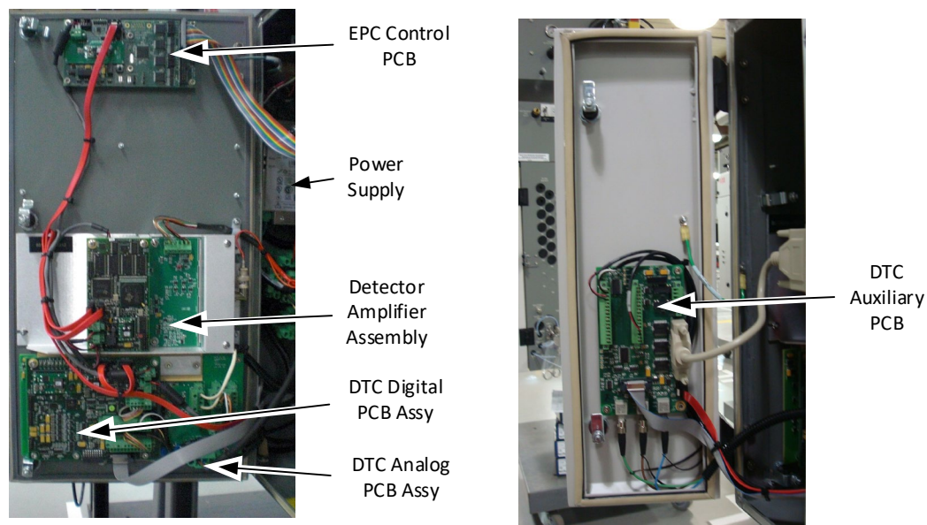
Fig. 6.4. Class B Oven Component Locations
