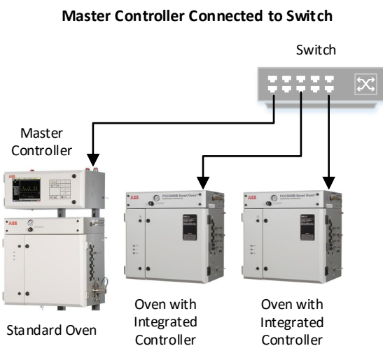
Figure 3.1. Standard PGC5000 with Ovens Connected by Switch
