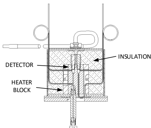
Fig. 9.2. Single Port TCD with Heater Block
