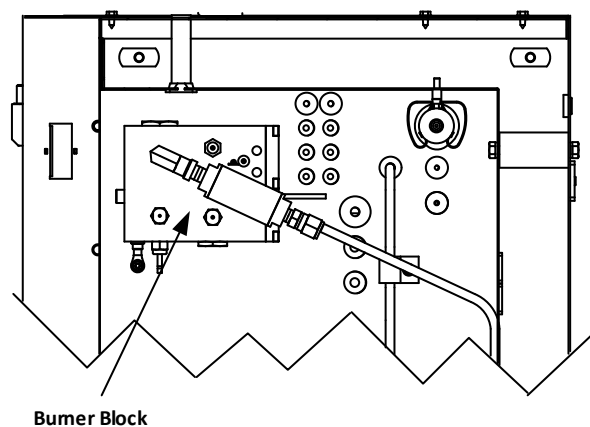
Fig. 7.6. Burner Block
