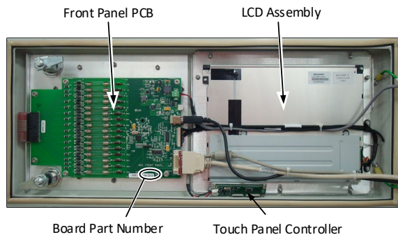
Fig. 6.3. Master Controller Front Door
