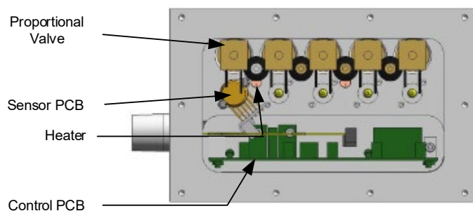
Fig. 8.16. EPC Control Assembly
