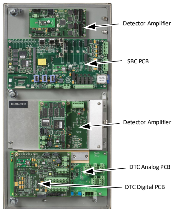
Fig. 6.6. Oven with Integrated Controller Component Locations
