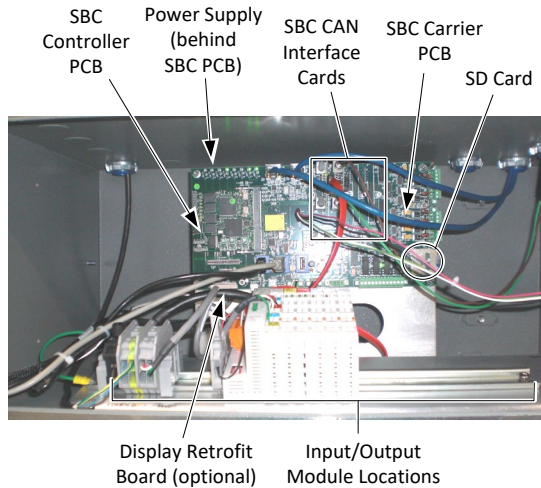
Fig. 6.1. Master Controller Component Locations
