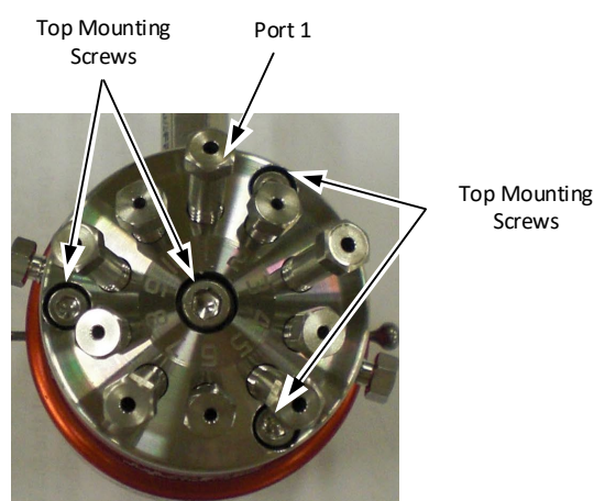
Fig. 7.17. Four-Screw Cap, Showing Port 1 Orientation
