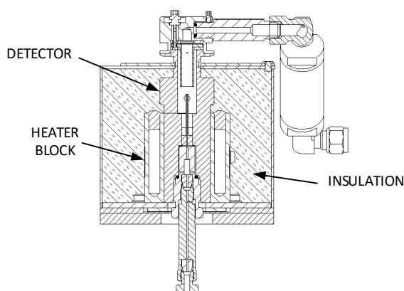
Fig. 9.1. FID with Heater Block
