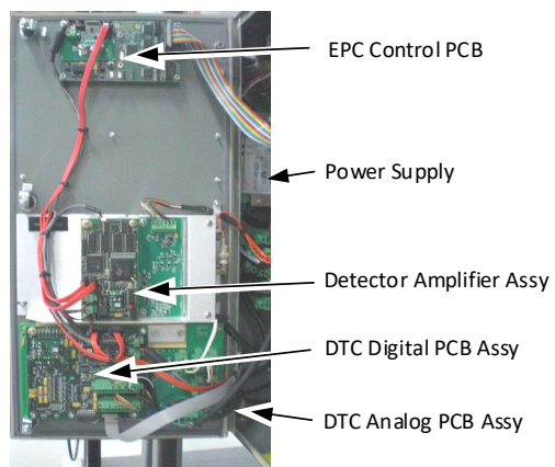
Fig. 8.6. Left Side Components
