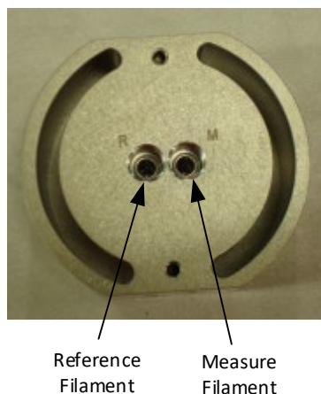
Fig. 8.11. Single-Port TCD Components
