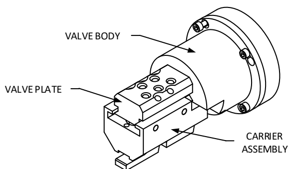
Fig. 7.12. Typical M2CP Valve
