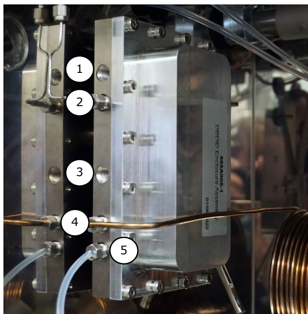
Fig. 8.15. DID Replacement Parts
