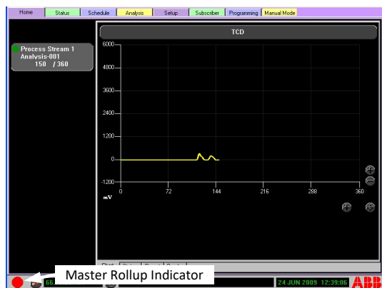
Fig. 5.5. Master Rollup Indicator Location
