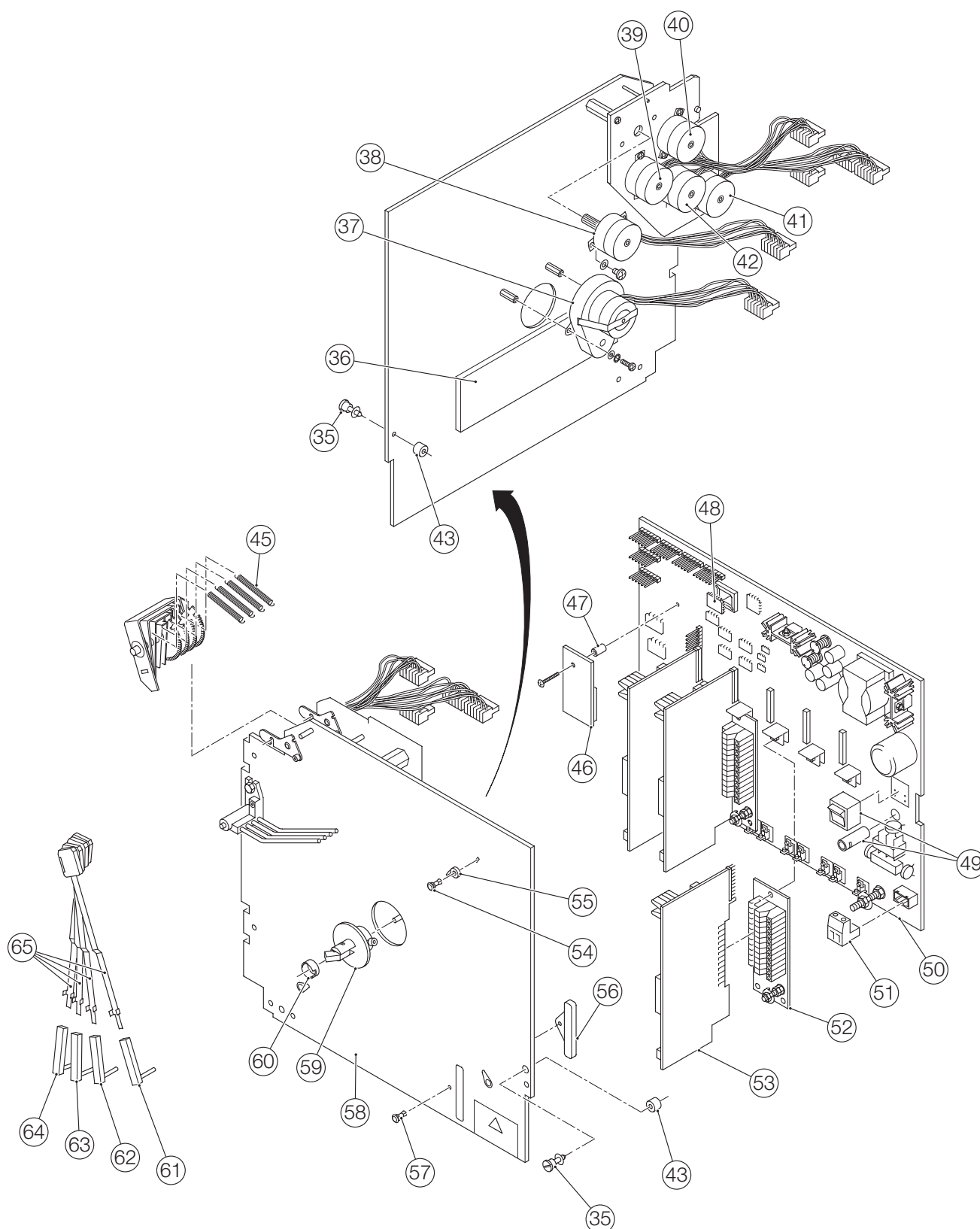
Figure 2 Replacement parts list – internal components
