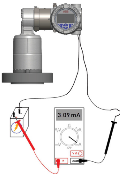
Figure 2 LLT100 current measurement
