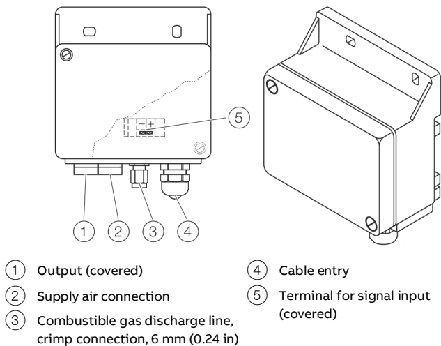
Figure 8: Plastic field mount housing
