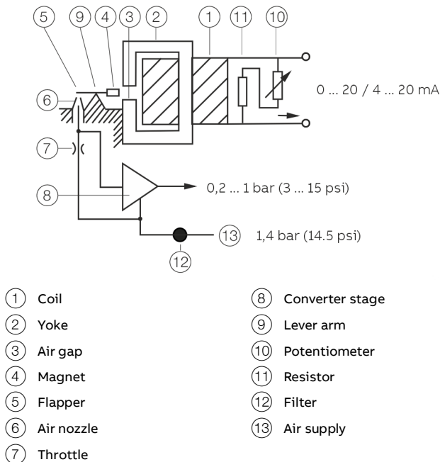
Figure 1: Schematic structure
