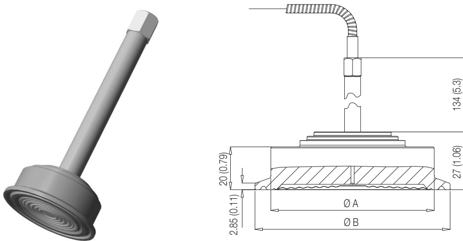
Figure 20: Triclamp sanitary seal
