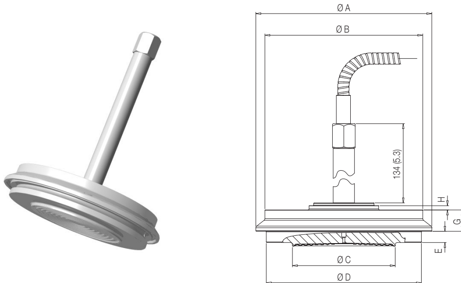
Figure 21: Cherry Burrell sanitary seal
