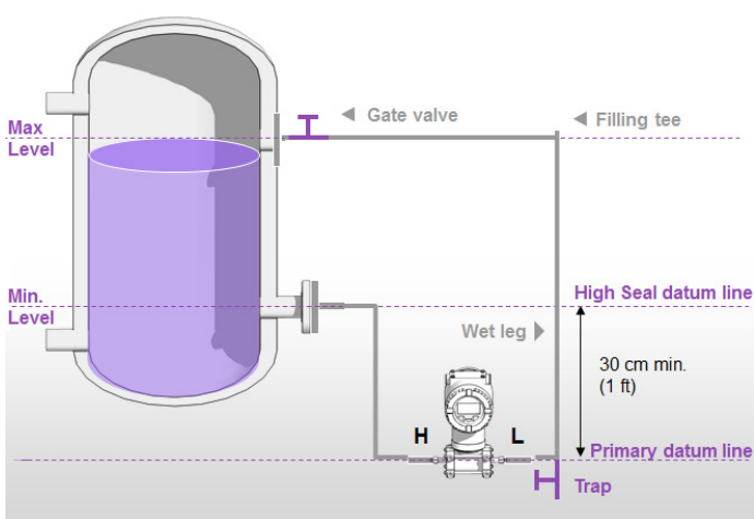
Figure 39: Level measurement of a liquid in a closed tank - vacuum or pressure service - wet leg installation
