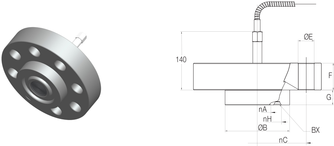
Figure 4: Flush rotating-flange (API) ring-joint construction
