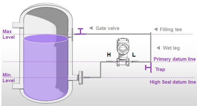
Figure 38: Level measurement of a liquid in a closed tank - pressure service only - wet leg installation
