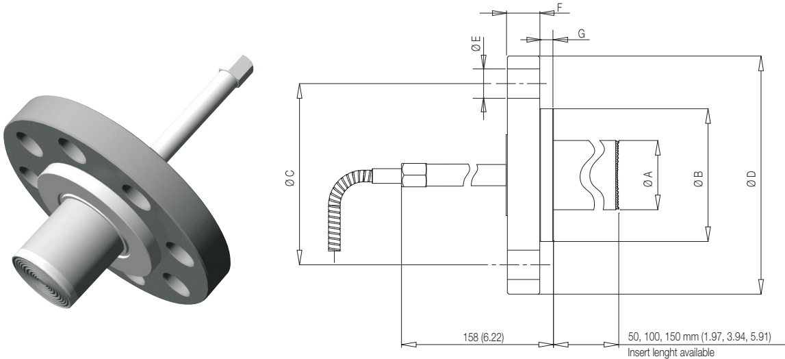
Figure 3: Extended rotating-flange seals
