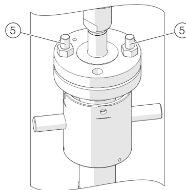
Figure 39: Screwing in the flange screws
