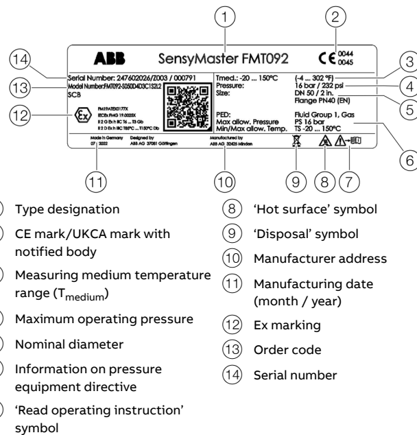
Figure 11: Pipe component name plate
