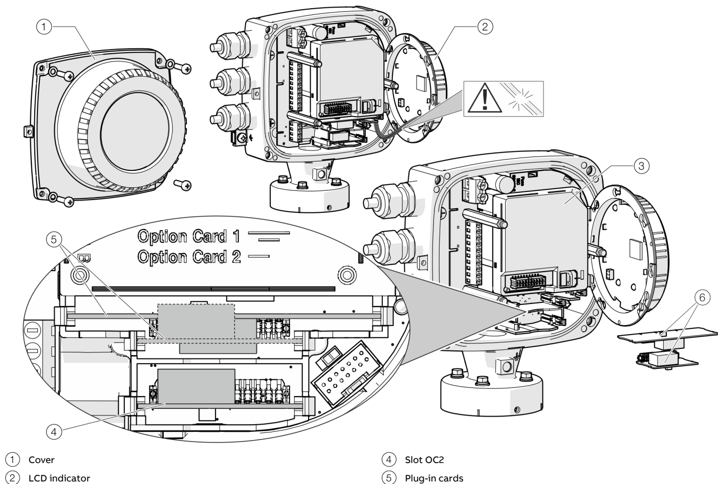
Figure 51: Installation of plug-in cards (example, single-compartment housing)
