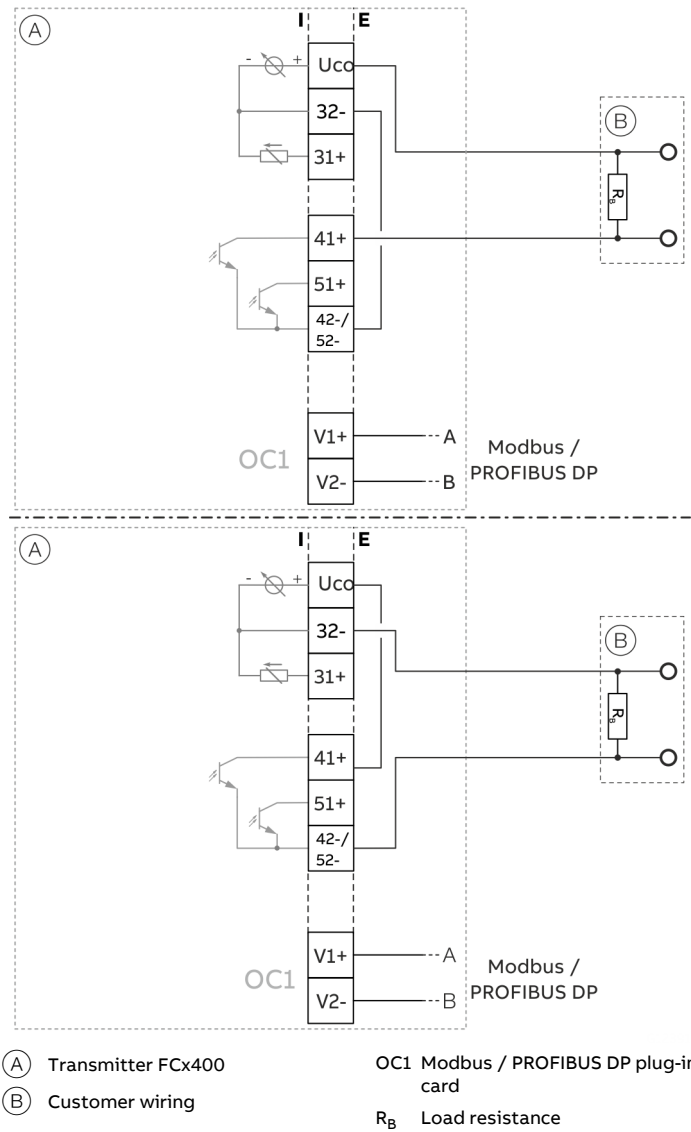
Figure 56: Current output Uco / 32 in power mode
