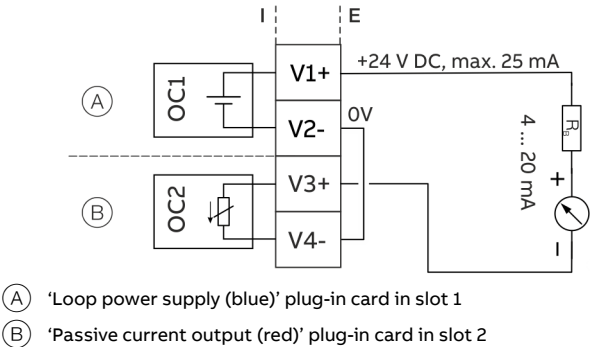
Figure 68: Active current output V3 / V4 (example)
