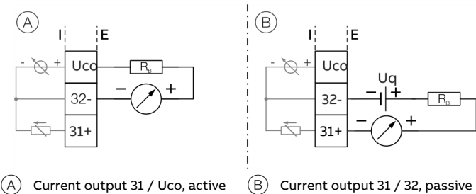
Figure 54: (I = internal, E = external, R_B = load)
