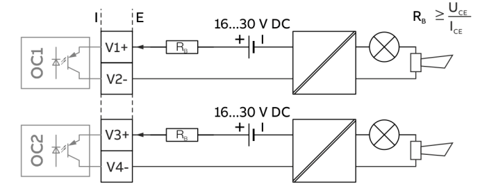
Figure 62: Plug-in card as binary output (I = internal, E = external, RB = load)
