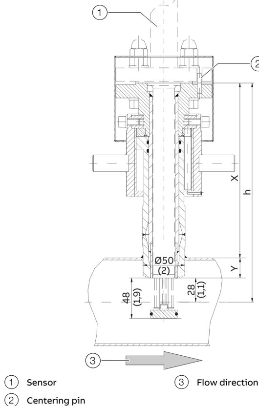
Figure 28: Integrated hot tap fitting in measurement position, dimensions in mm (in)
