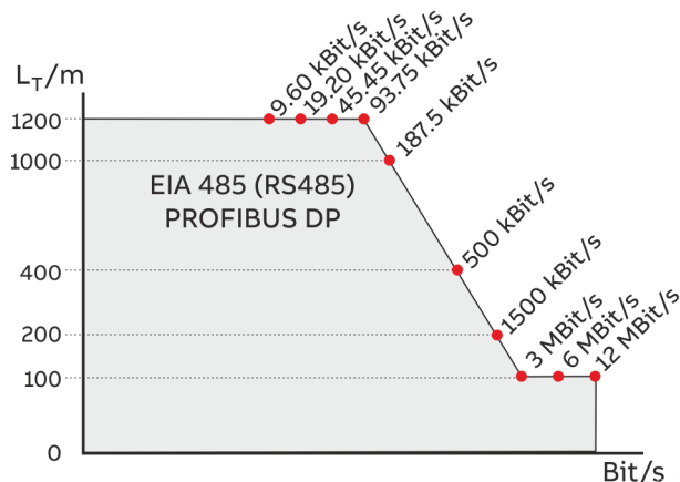
Figure 76: Bus cable length depends on the transmission rate
