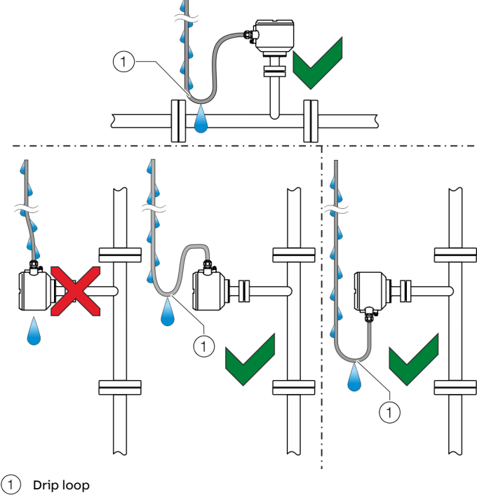
Figure 52: Laying the connection cable
