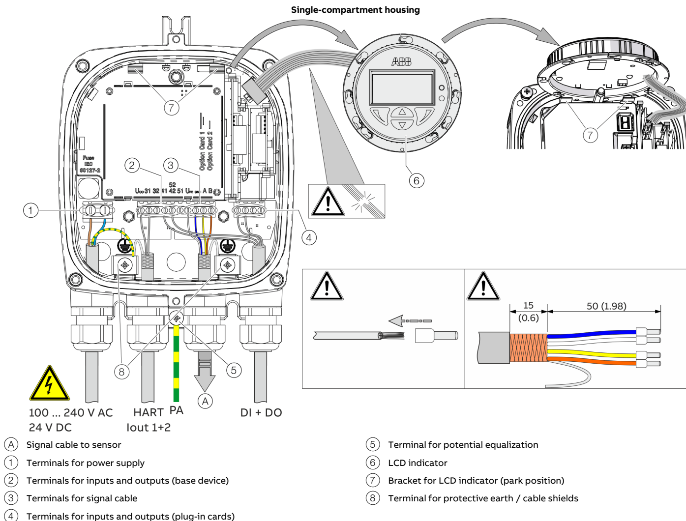
Figure 73: Electrical connection to transmitter in remote mount design [example, dimensions in mm (in)]
