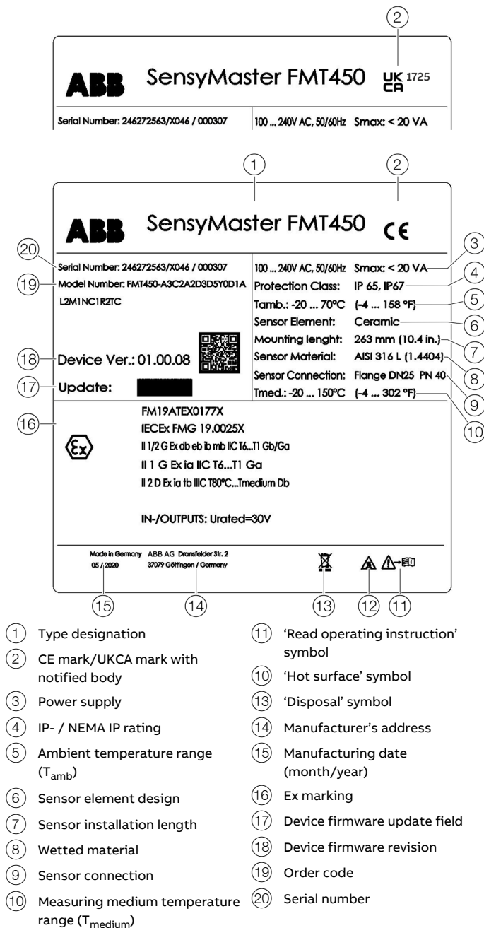
Figure 10: Name plate (example)
