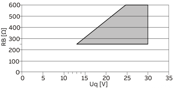
Figure 54: (I = internal, E = external, R_B = load)
