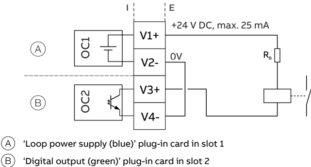
Figure 66: Active digital output V3 / V4 (example)
