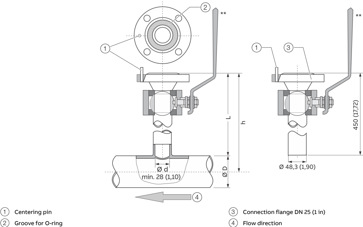
Figure 22: Dimensions in mm (in)
