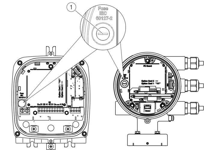
1 Fuse holder
