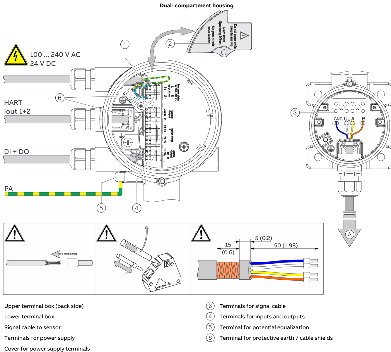
Figure 72: Electrical connection to transmitter in remote mount design [example, dimensions in mm (in)]
