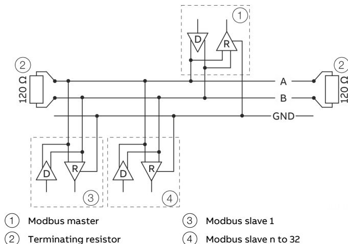
Figure 75: Communication with the Modbus protocol
