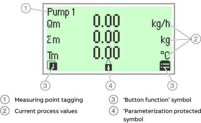
Figure 88: Process display (example)
