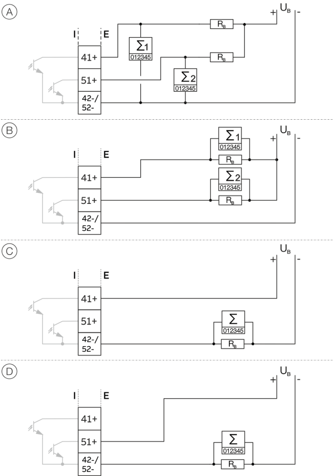
Figure 70: Connection versions digital output 41 / 42 and 51 / 52
