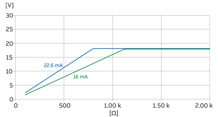
Figure 57: Output voltage dependent on load resistance
