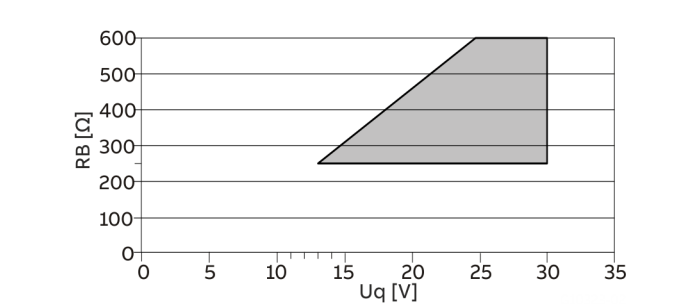
Permissible source voltage U_q for passive outputs in relation to load resistance R_B where I_{max} = 22\text{ mA} . = Permissible range
