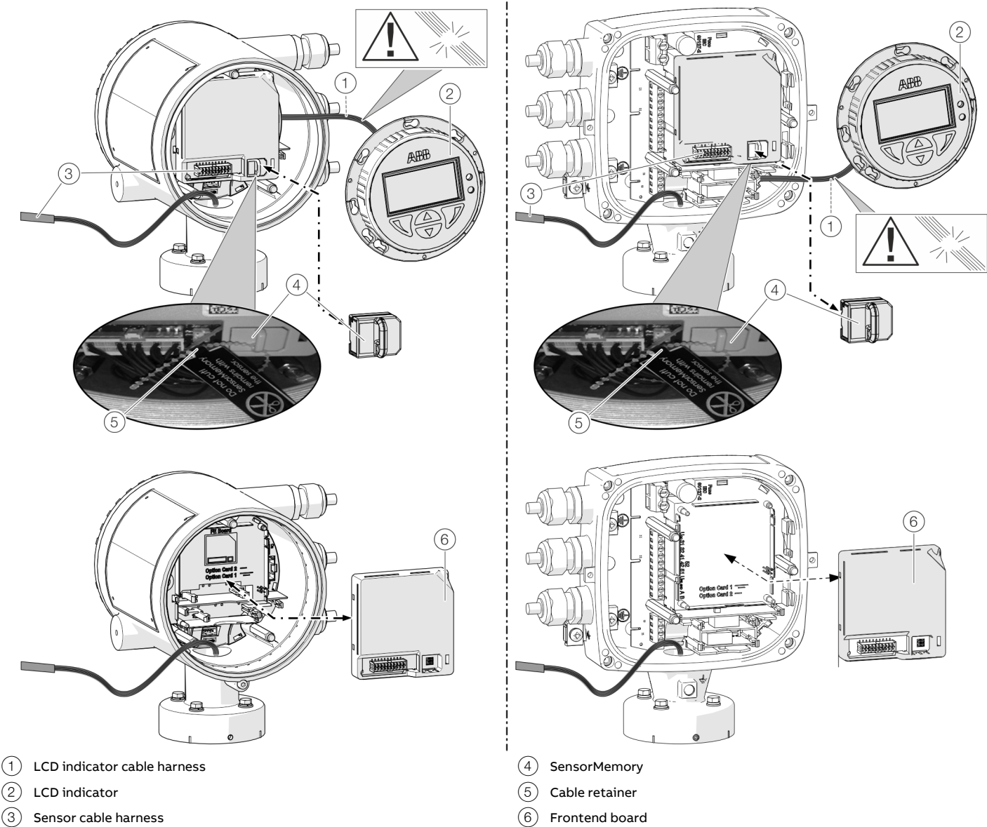
Figure 93: Replacing LCD indicator and frontend board (example)
