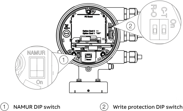
Figure 77: Position of the DIP switches
