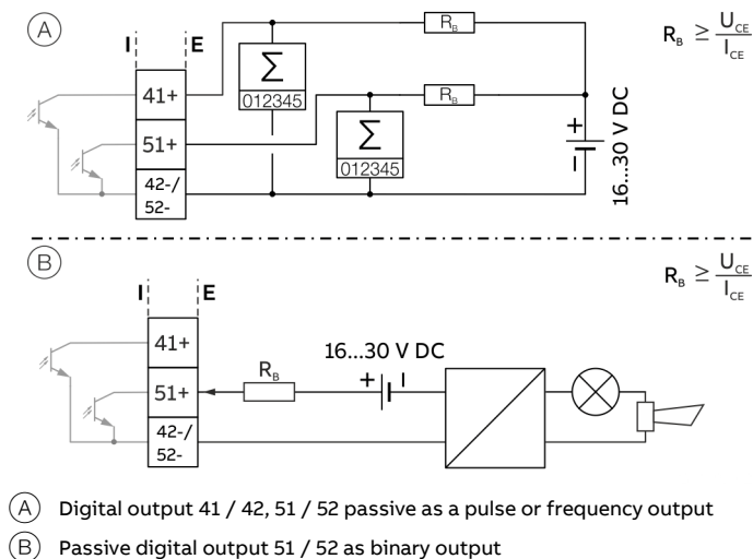
Figure 58: (I = internal, E = external, R_B = load)
