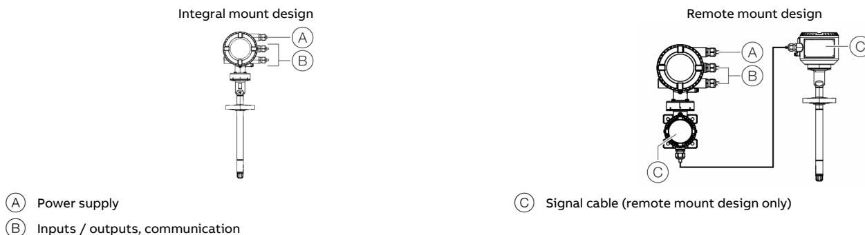
Figure 1: Electrical connections overview
