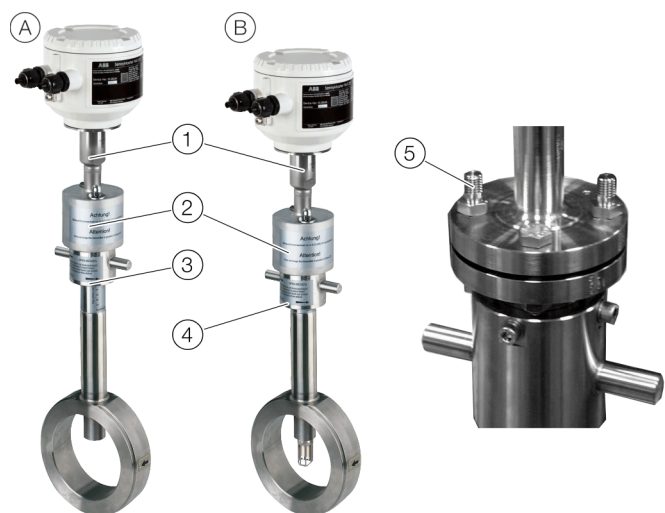
Figure 30: Sensor connection on the hot tap fitting
