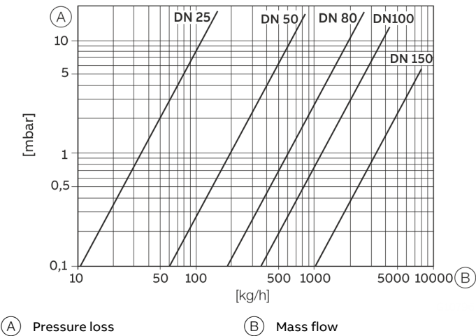
Figure 16: Pressure loss in logarithmic representation
