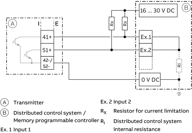
Figure 67: Digital output 41 / 42 on distributed control system (example)
