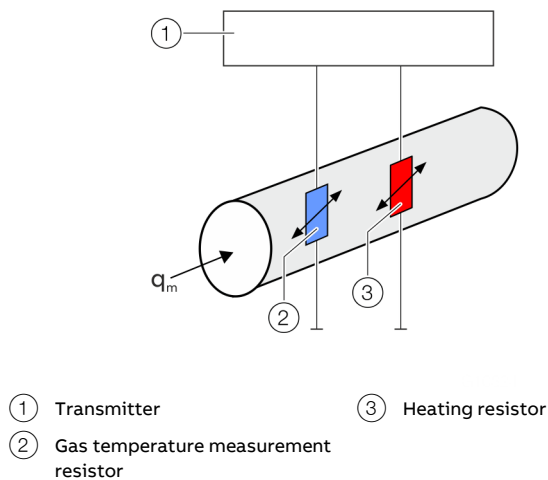
Figure 9: Measuring principle (simplified)
