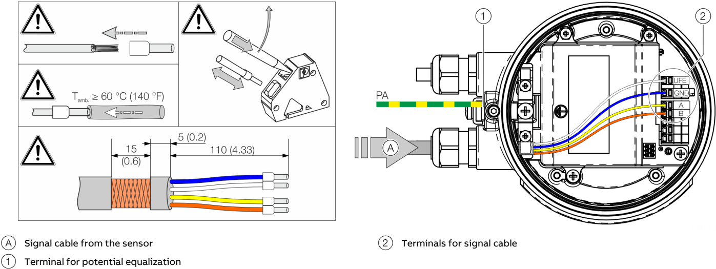
Figure 74: Connection to sensor in remote mount design (example)
