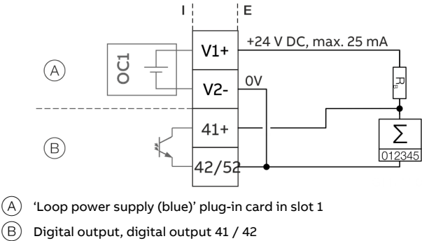
Figure 65: Active digital output 41 / 42 (example)
