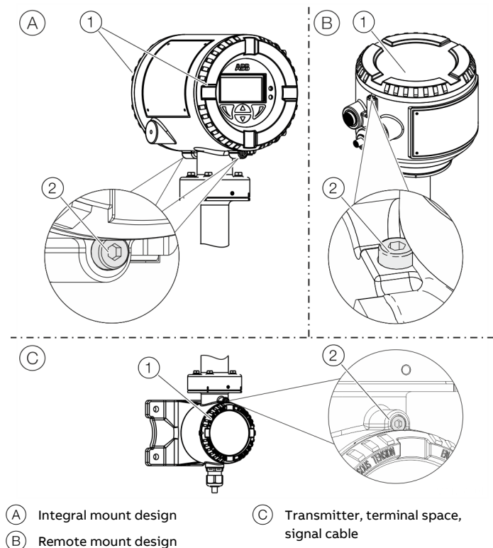
Figure 45: Cover lock (example)
