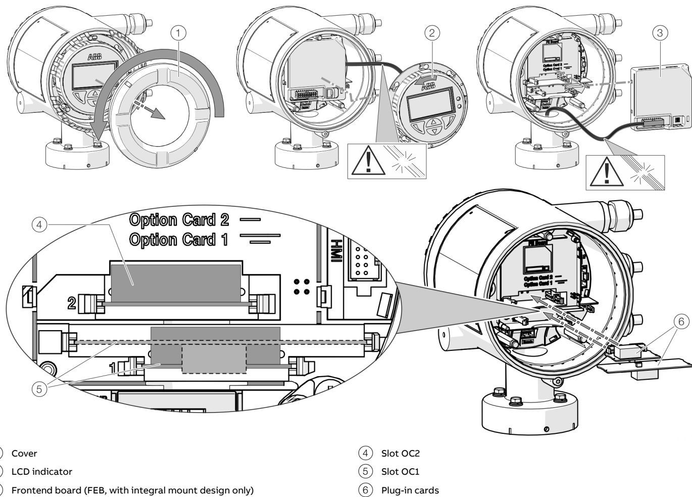
Figure 50: Installation of plug-in cards (example, dual-compartment housing)
