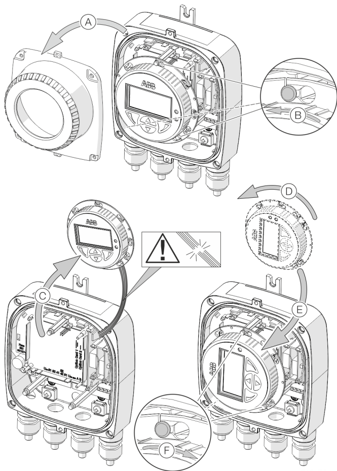
Figure 49: Rotating the LCD indicator
