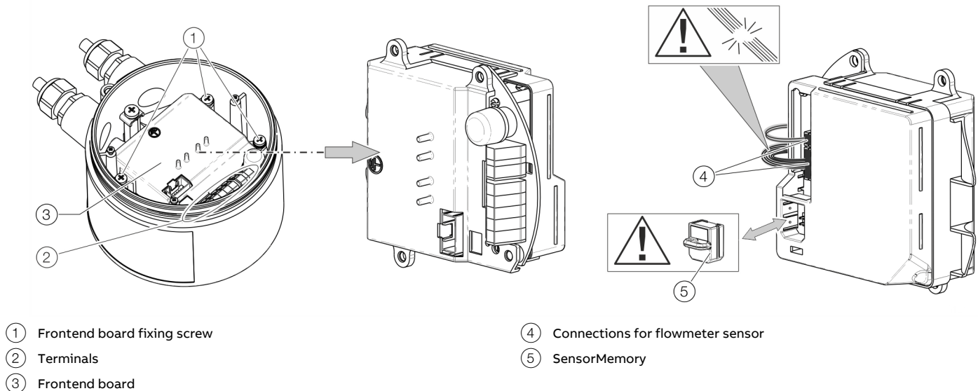
Figure 94: Replacing the frontend board (flowmeter sensor)
