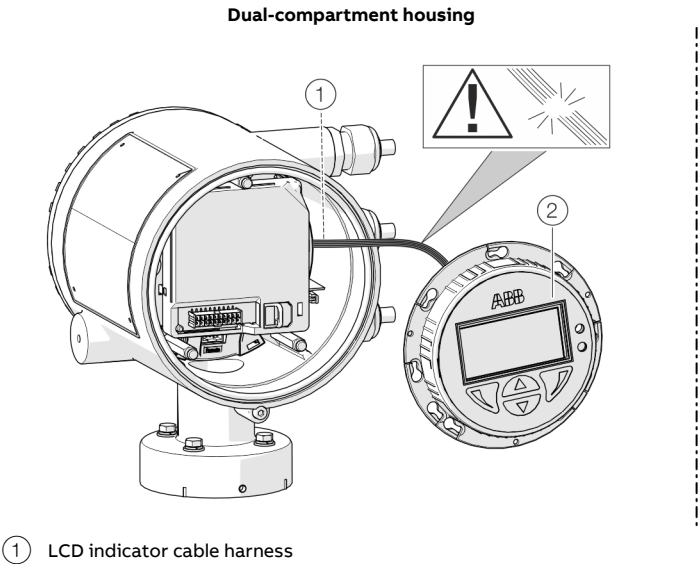
Figure 92: Replacing the LCD Indicator (example)
