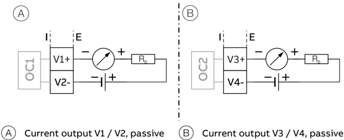
Figure 60: (I = internal, E = external, RB = load)
