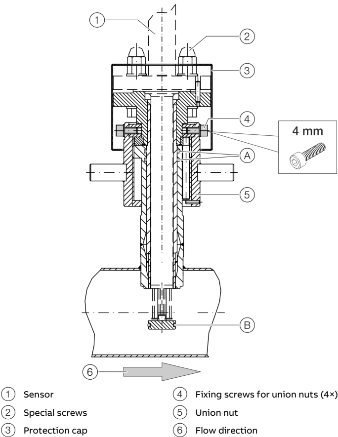
Figure 90: Gaskets on the hot tap fitting
