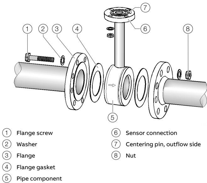
Figure 19: Installing a pipe component (example, wafer type design)
