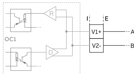
Figure 59: Plug-in card as a Modbus / PROFIBUS DP interface (I = internal, E = external)
