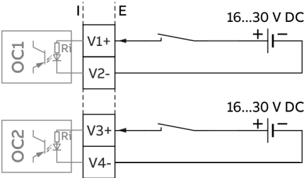
Figure 63: Plug-in card as digital input (I = internal, E = external)
