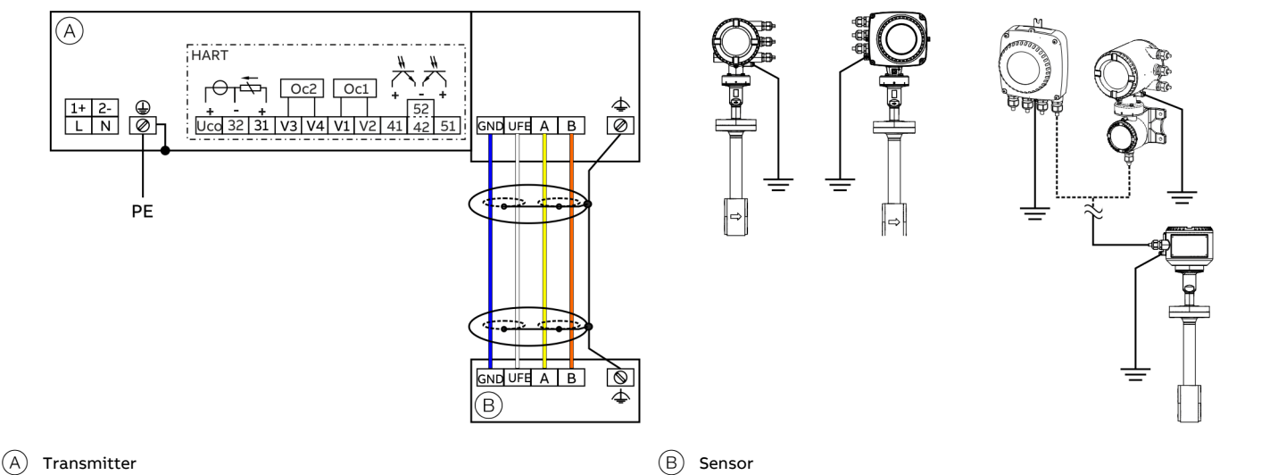
Figure 53: Electrical connection
