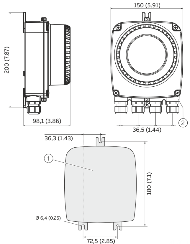
Figure 43: Assembly set for 2" pipe mounting
