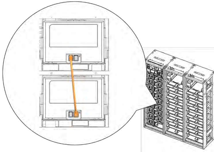
Figure 3-97: Module #4 to Module #5 Signal Cabling
