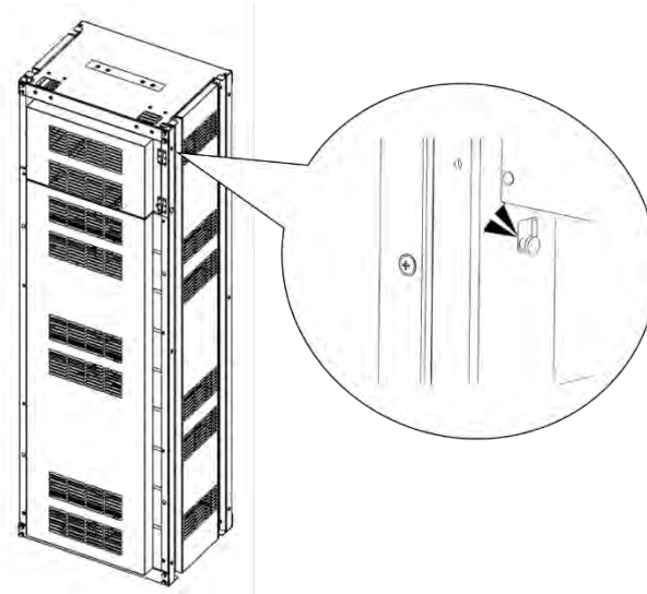
Figure 3-8: Side panel hooks (four)
