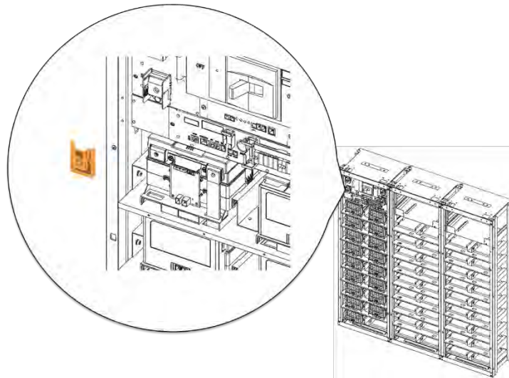
Figure 3-90: Remove SMU B+ Terminal Cover
