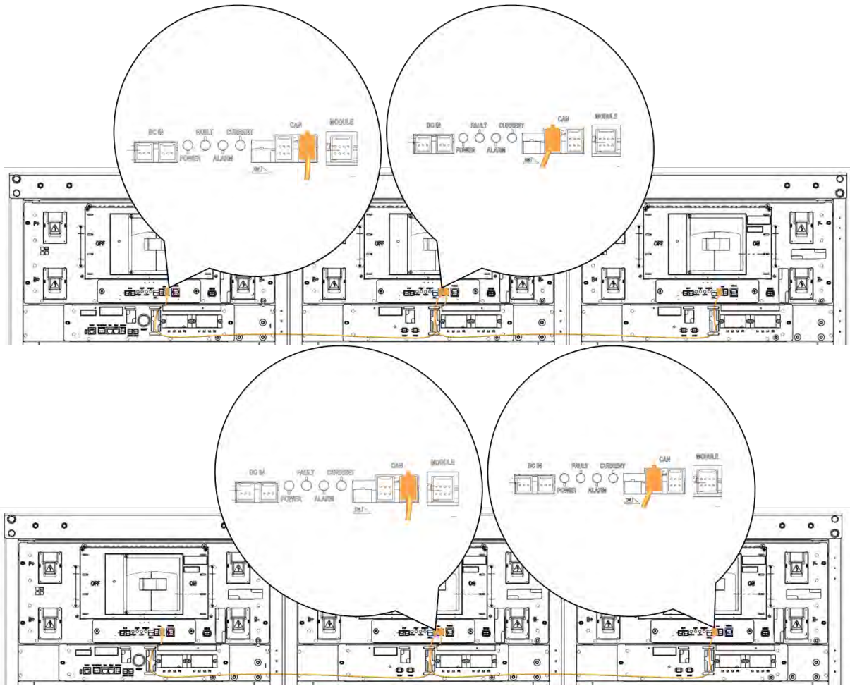
Figure 3-111: Signal Cabling Examples of Left Alignment of SMU
