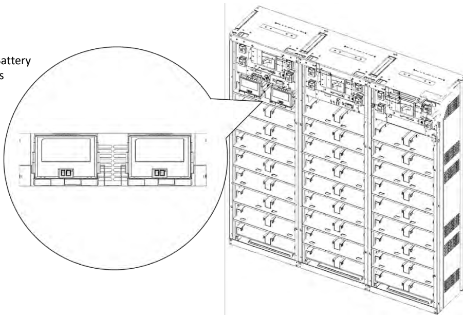
Figure 3-25: Insertion of Modules on the Ninth Shelf from the Bottom
