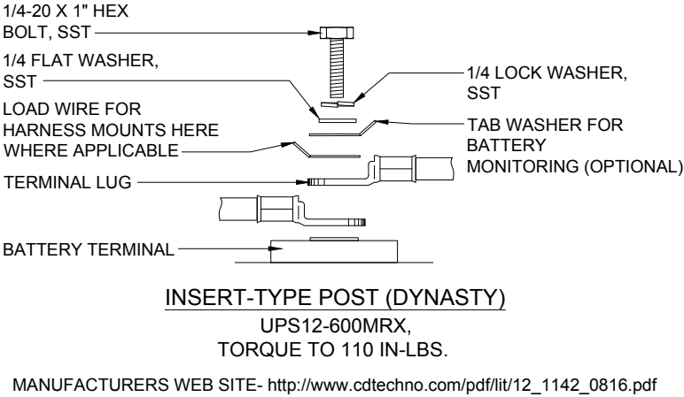
DETAIL 'A' REF: SHEET 4
