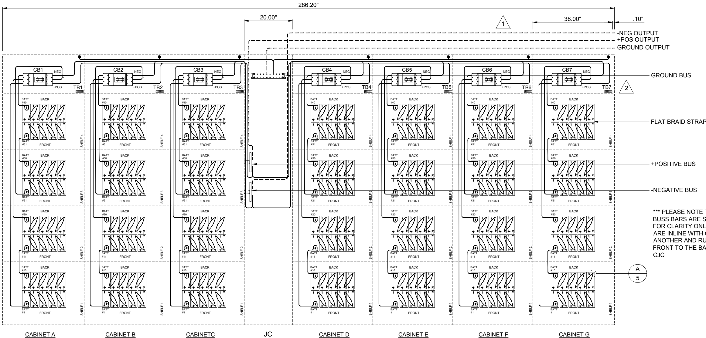
ELECTRICAL ILLUSTRATION
