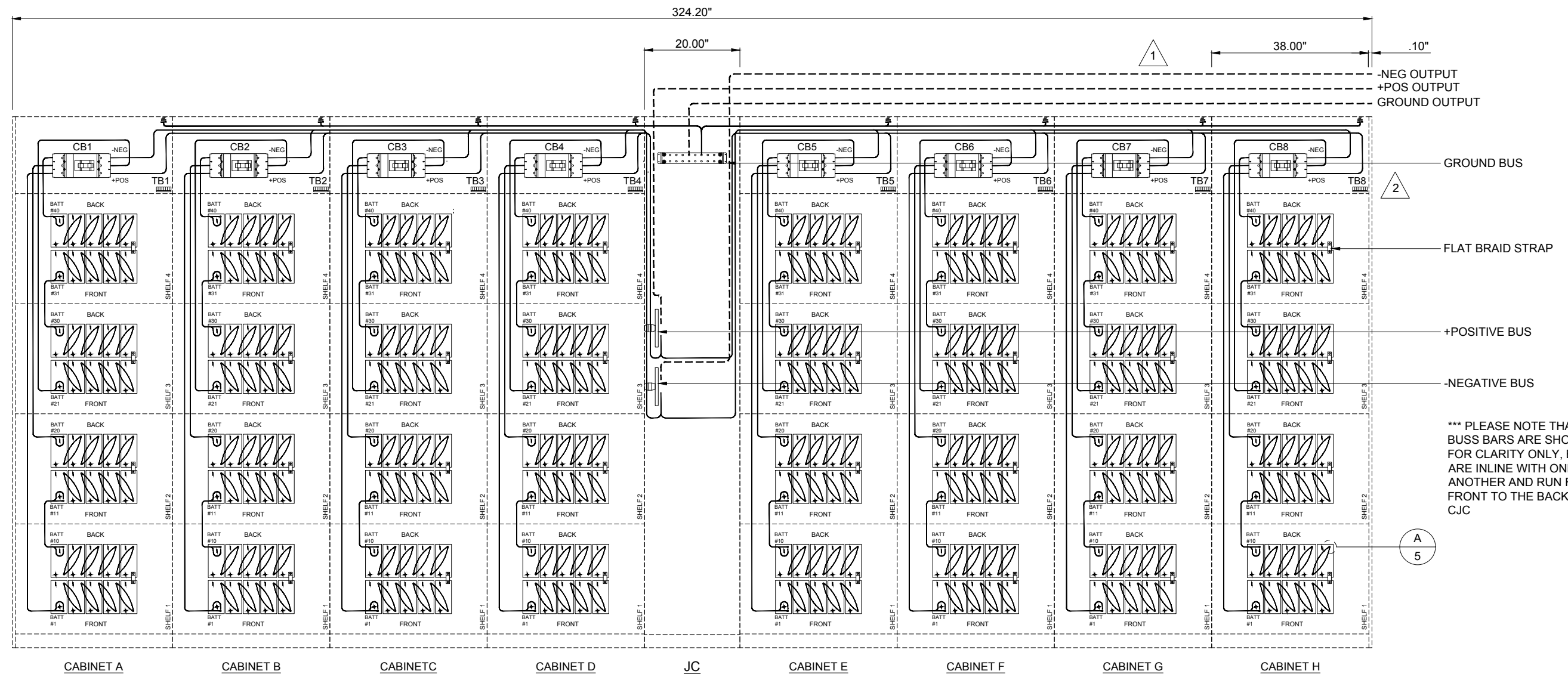
ELECTRICAL ILLUSTRATION
