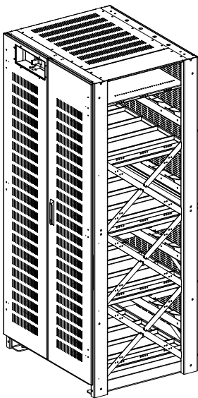
CABINET D
