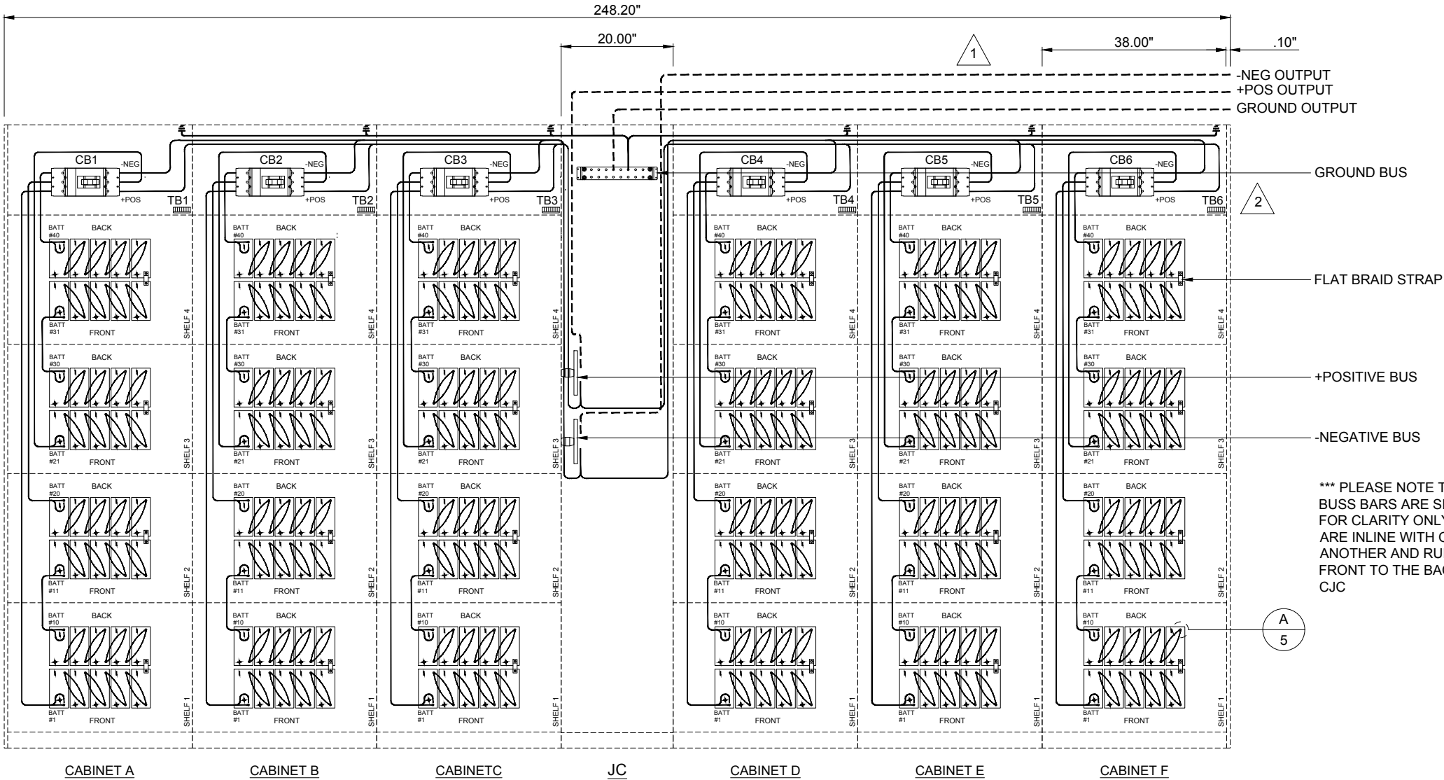
ELECTRICAL ILLUSTRATION
