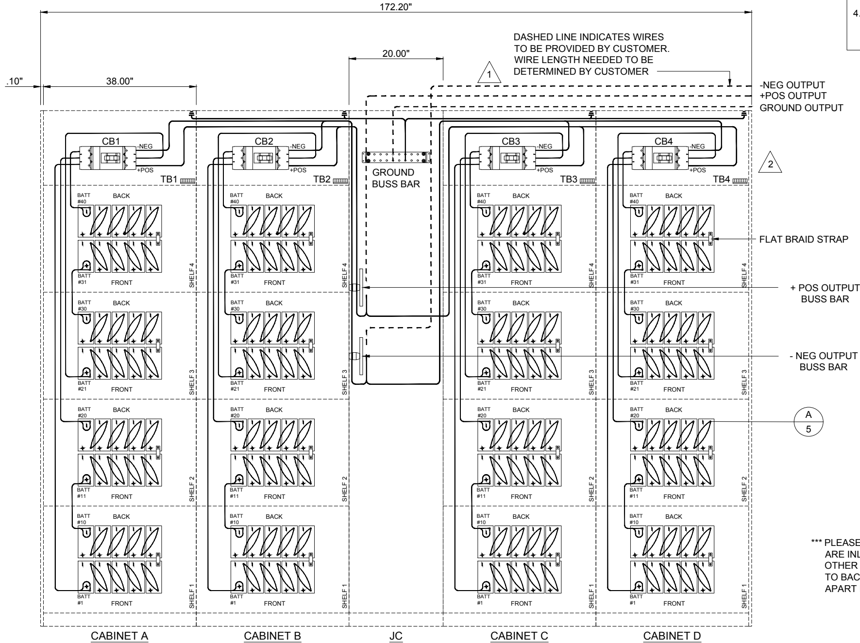
ELECTRICAL ILLUSTRATION
