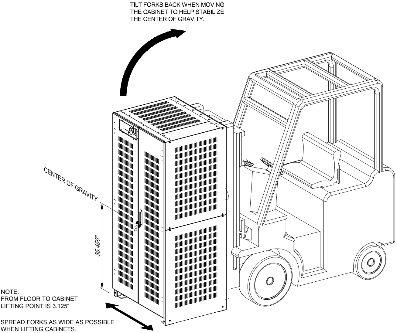
MOVING A BATTERY CABINET DO NOT LIFT THE CABINET HIGHER THAN NECESSARY TO CLEAR THE FLOOR WHEN MOVING
