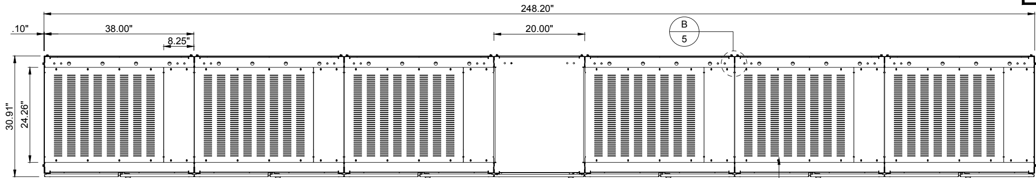
TOP VIEW
