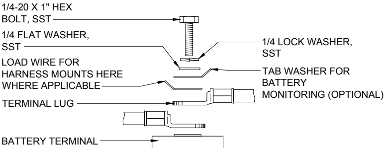
INSERT-TYPE POST (DYNASTY) UPS12-600MRX, TORQUE TO 110 IN-LBS.
