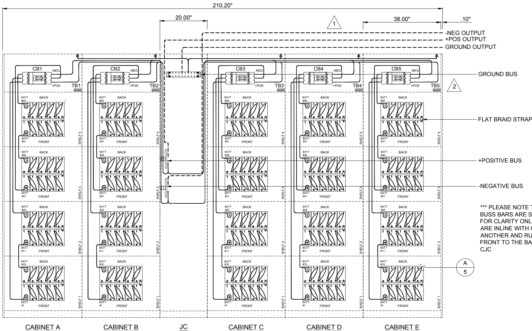
ELECTRICAL ILLUSTRATION
