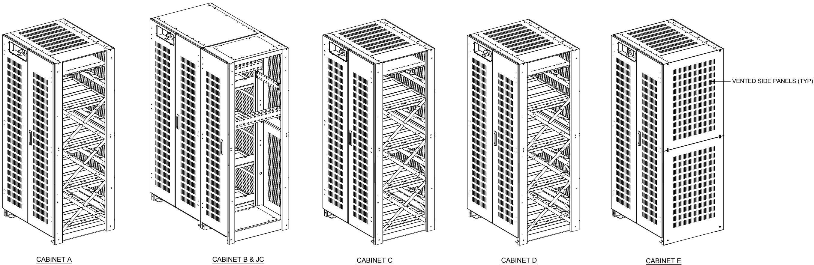
ISOMETRIC BATTERY CABINET VIEW
