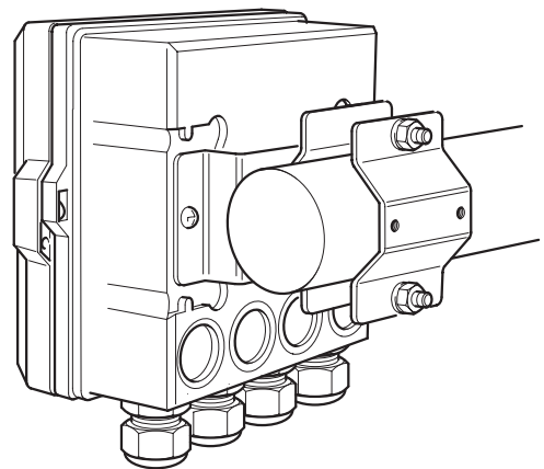
Horizontal pipe-mount
