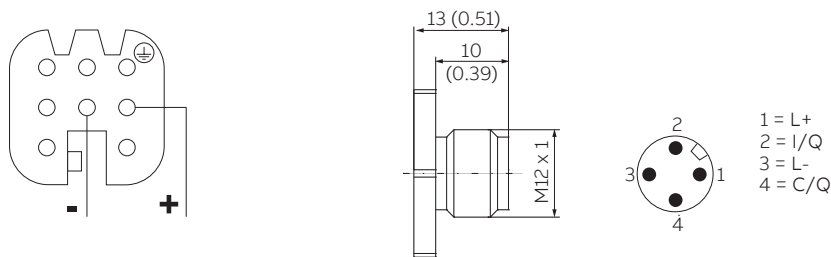
Figure 17 Pin layout of Harting HAN 8D (socket view) and M12 x 1 connector - IO-Link, 4-pin, A-encoded
