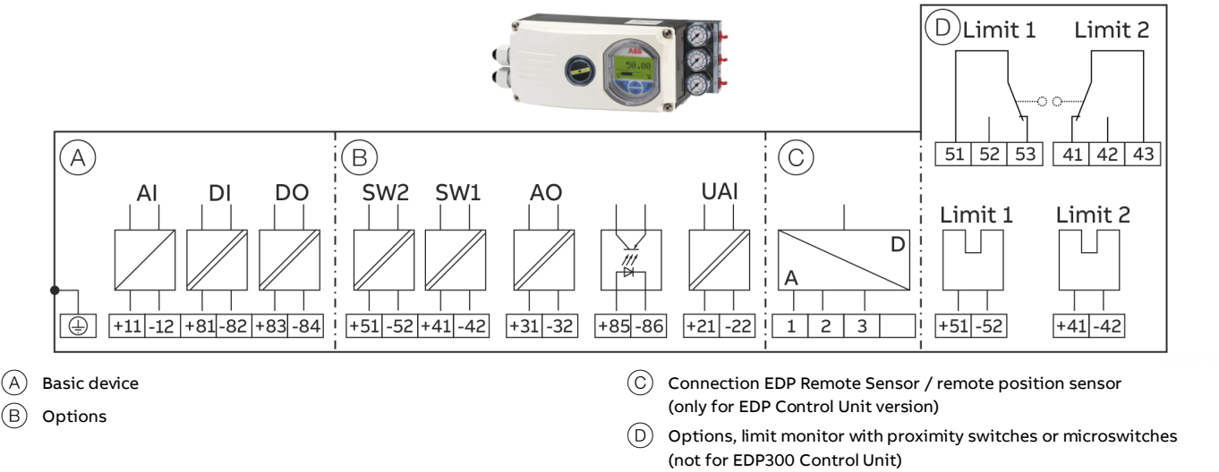
Figure 15: EDP300 Electrical Connection
