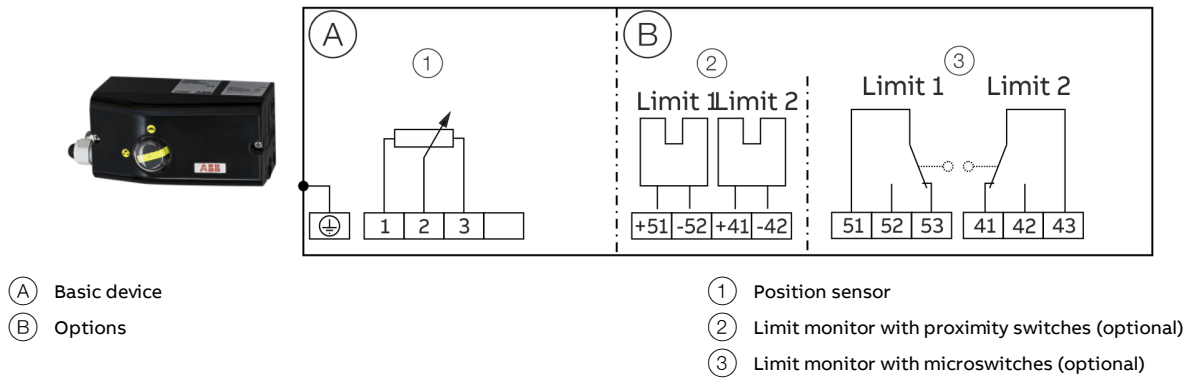
Figure 16: EDP300 Remote Sensor Electrical Connection
