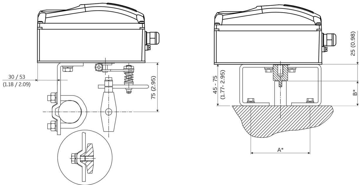
Figure 19: Mounting to linear actuators to DIN/IEC 534
