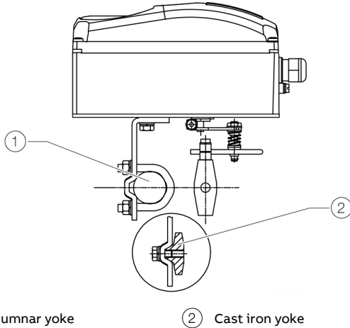
Figure 2: Mounting to linear actuators in accordance with DIN / IEC 534
