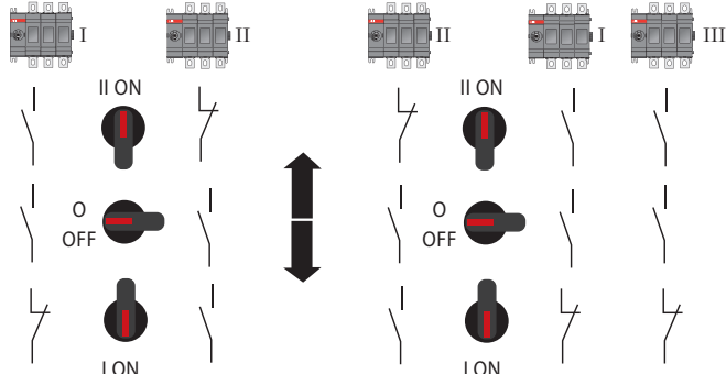
Change-over switches
