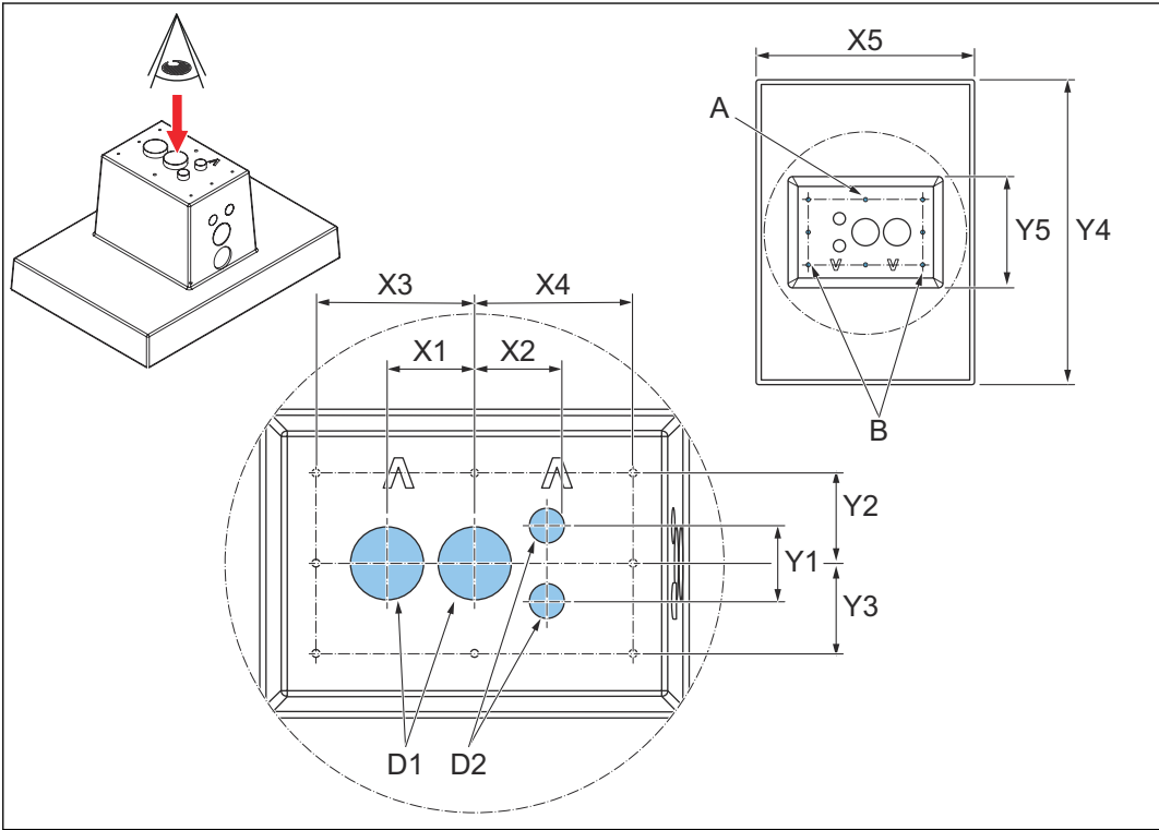
Dimensions, top view
