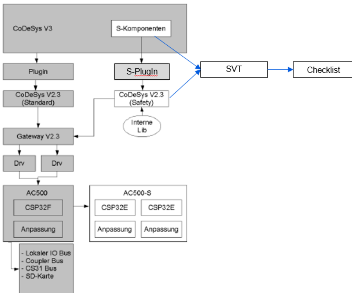
Figure 5: Overview of application development Tool
