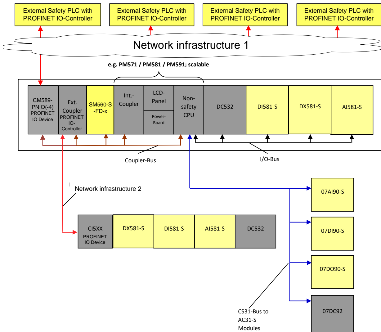
Figure 4: Extended overview of Safety PLC „SM560-S-FD-1/-4“ & non-safety components
