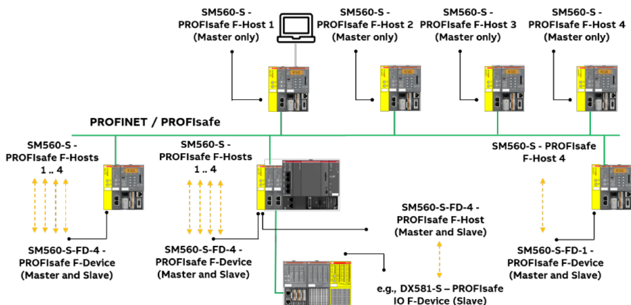
Figure 2: Safe CPU comm. between Safety CPUs (SM560-S / -FD1 / -FD4) (Example)
