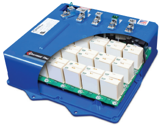
ISM™ – Integrated Suppression Module Individual thermally fused and protected MOV component of SL3™, TG3™ and PX3™ products.
