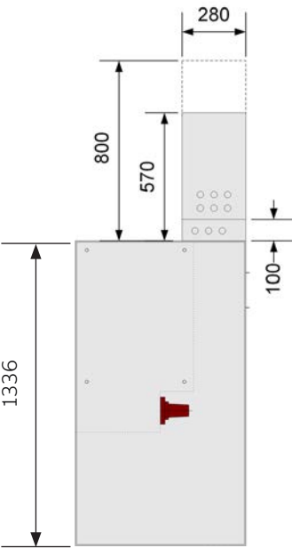
Low voltage compartment for V20/V25
