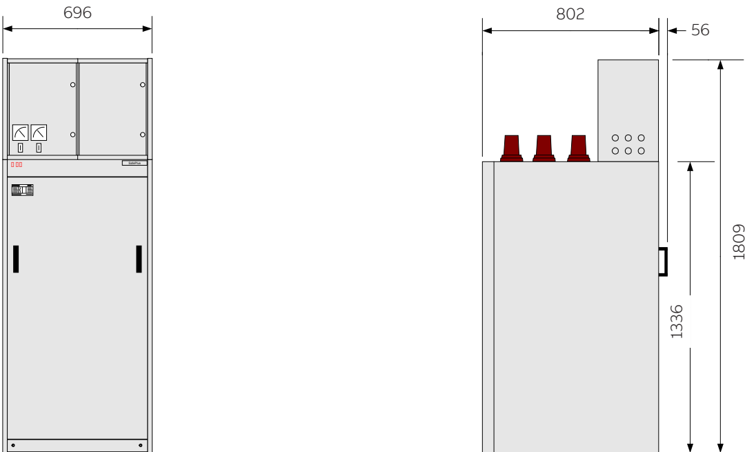
Metering module M, front view
