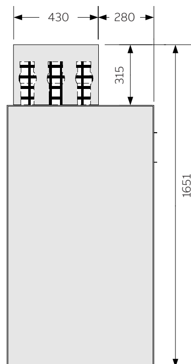
Busbar cover
