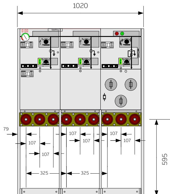
3-way (CCF-module)
