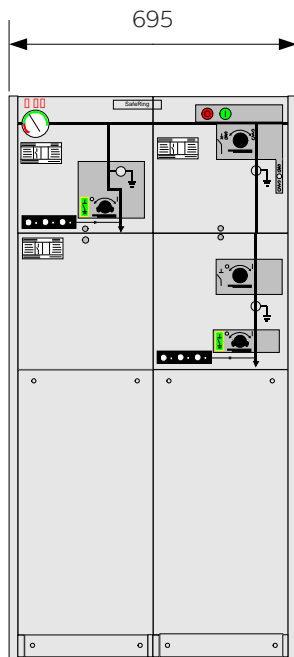
2-way (CV-module)
