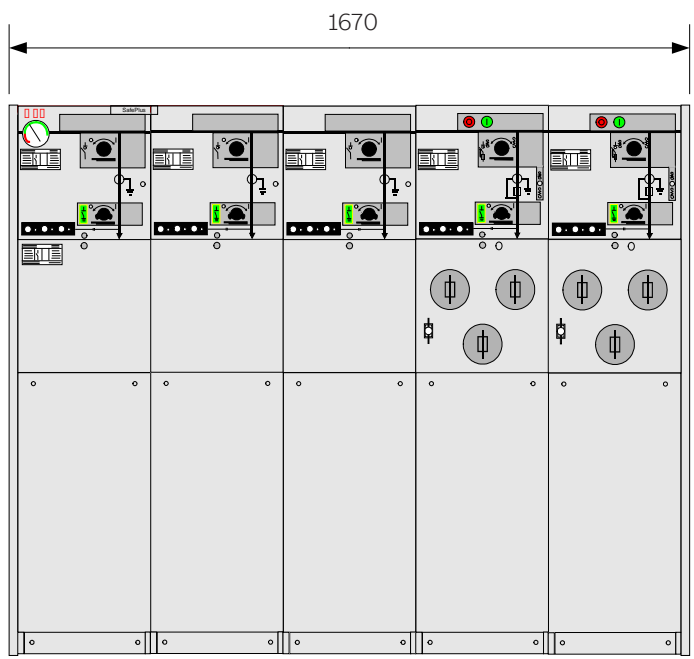
5-way (CCCCFF-module)
