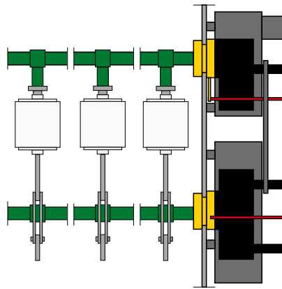
V-mechanism
