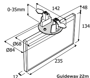
Guideway 22m
