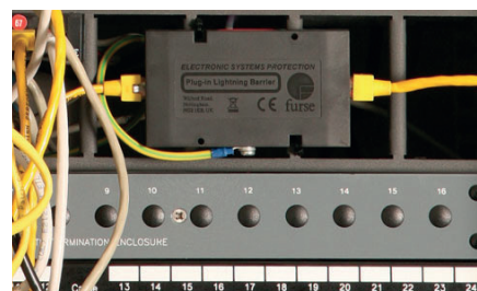
An ABB ESP Cat-6 (above and detail below) protecting a hub from transient overvoltages on a network connection with another building.
