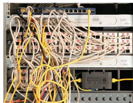
An ABB ESP Cat-6 (above and detail below) protecting a hub from transient overvoltages on a network connection with another building.
