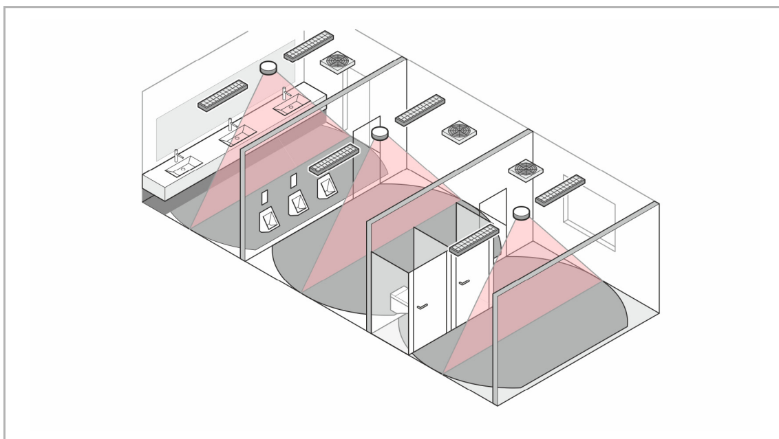
Fig. 25: Application example: DALI in a simple WC facility
