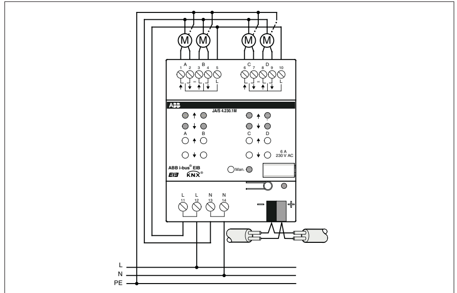
Diagram 15: Planning voltage monitoring in the circuits
