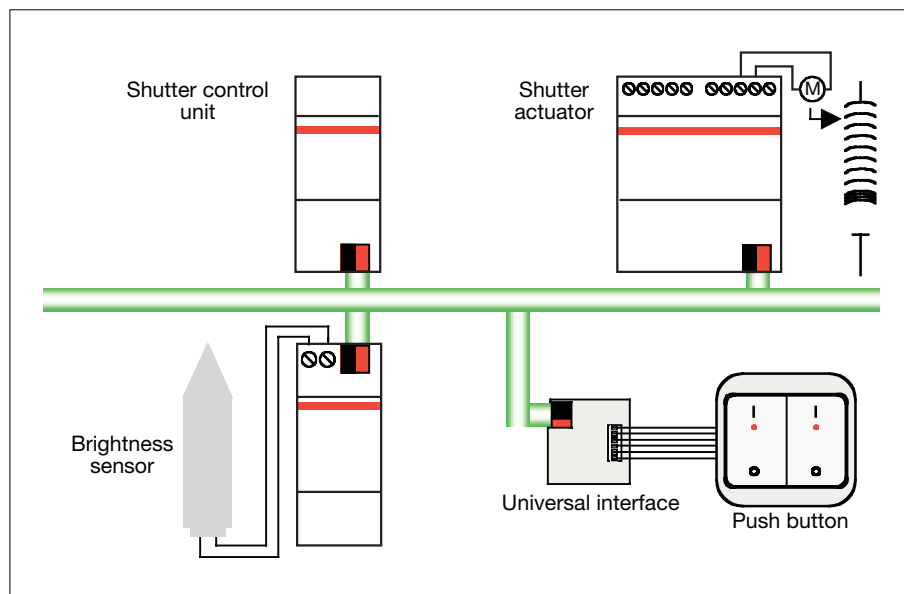
Diagram 11: Planning an automatic sun protection system with tracking of the sun's position
