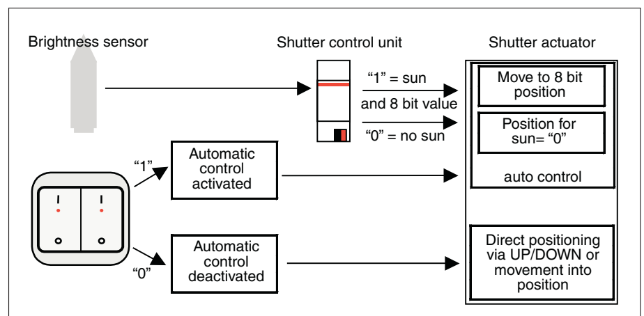
Diagram 10: Setting up an automatic sun protection system with tracking of the sun's position
