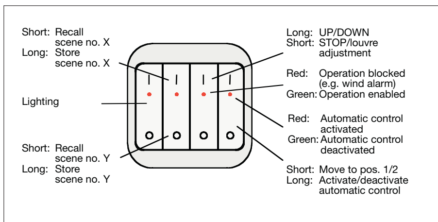
Diagram 17: Push button assignment UP/DOWN, move to position, automatic control
