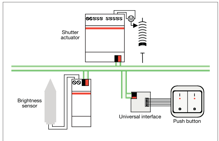
Diagram 9: Planning a simple automatic sun protection system
