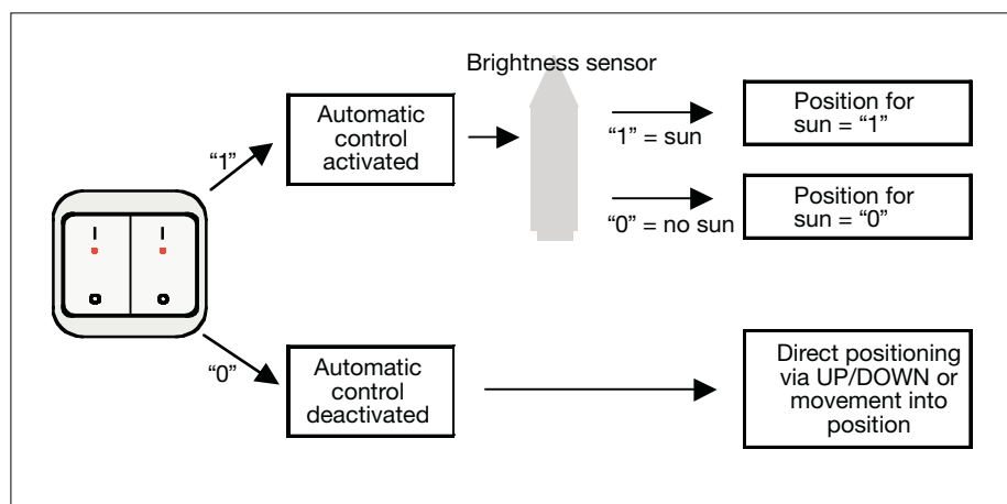
Diagram 8: Setting up a simple automatic sun protection system
