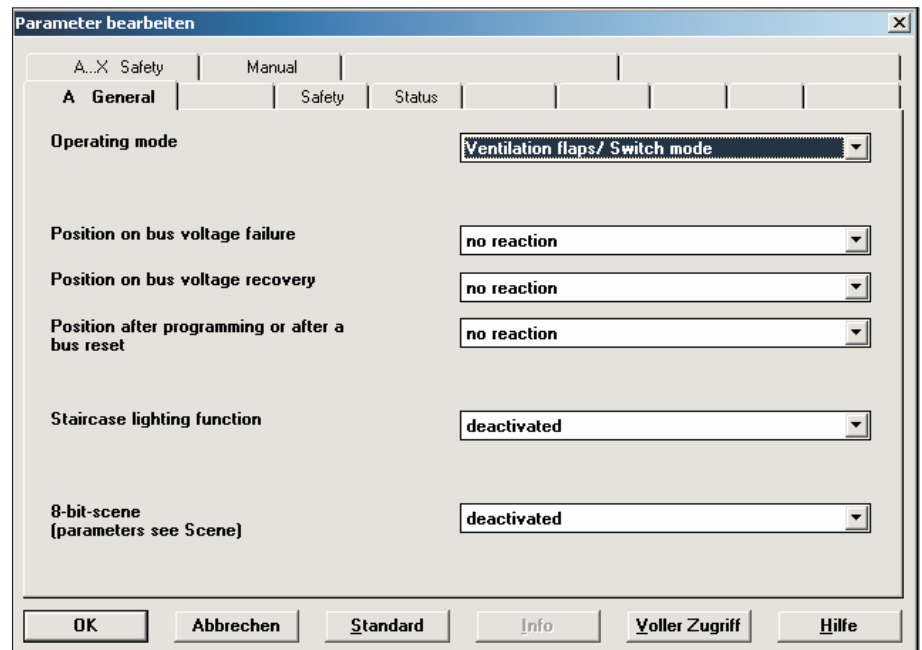
Diagram 37: “A - General” operating mode (operating mode “Ventilation flaps/switch mode”)
