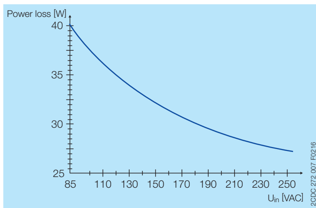
Typical power loss over AC input voltage
