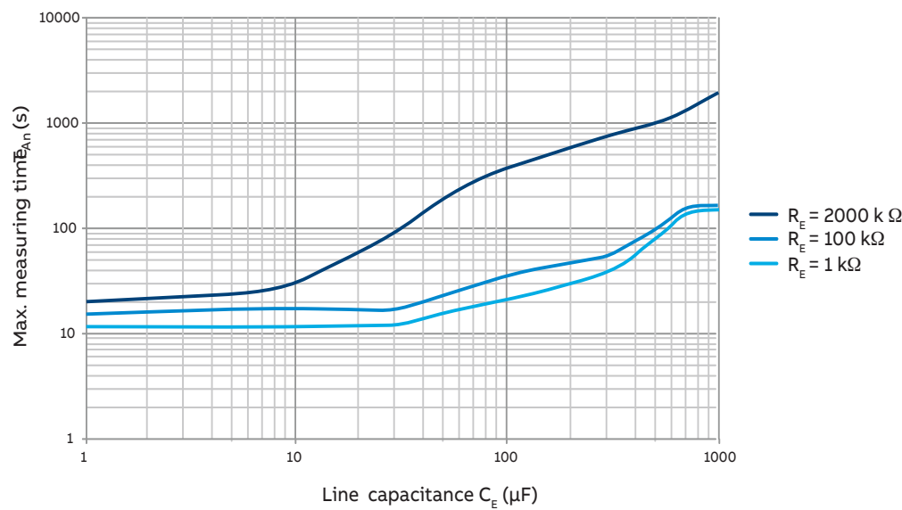
Max. measuring times in response to the line capacitance
