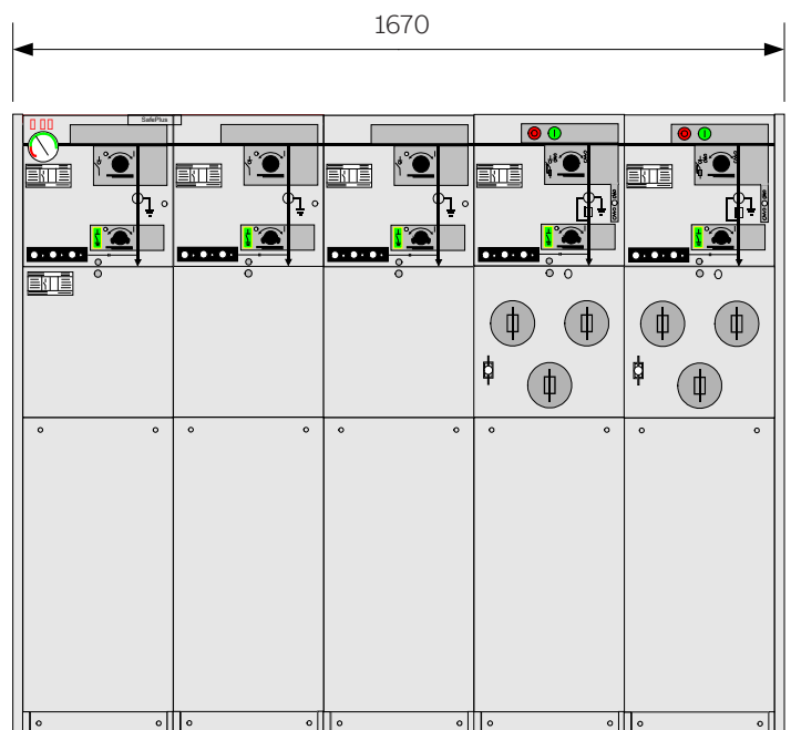
5-way (CCCFF-module)
