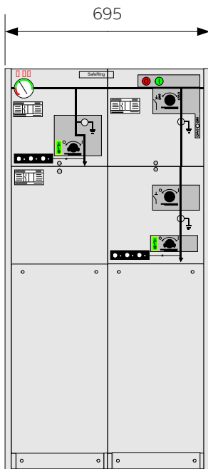
2-way (CV-module)
