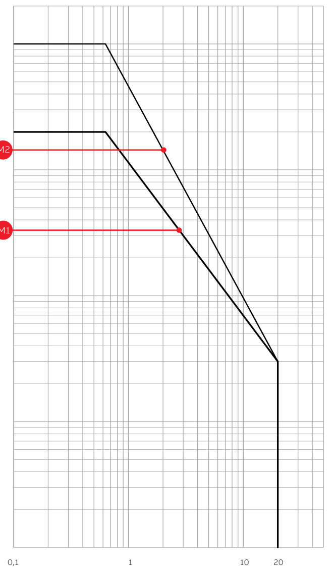
SafePlus V25 High duty - 15, 17,5 and 24kV (VG4 - M1/M2)
