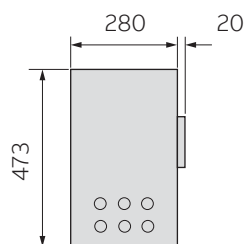
LVC with REF542plus
