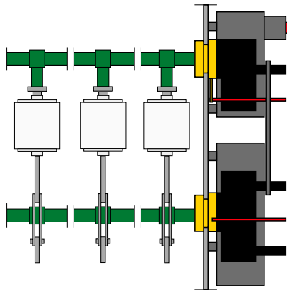
V-mechanism
