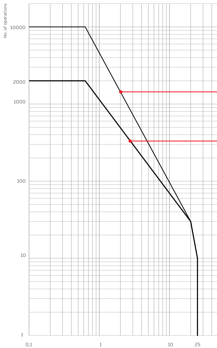
SafePlus V25 High duty - 12kV (VG4 - M1/M2)
