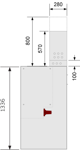
Low voltage compartment for V20/V25
