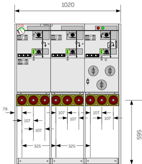
3-way (CCF-module)
