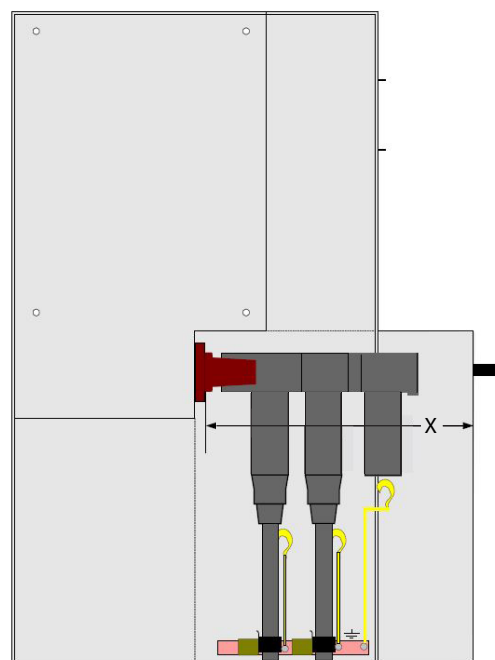
Extended cable cover with double cable and surge arrester
