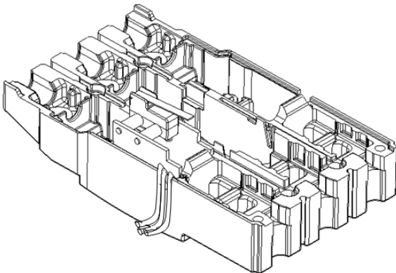
Figure 8. Auxiliary Switch, Left Pole Mounting
