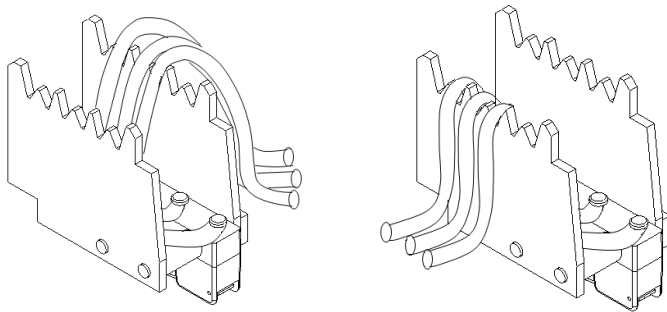
AUXILIARY SWITCH, RIGHT POLE
