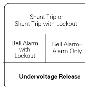
Figure 2. Accessory compartment on front of circuit breaker, with Undervoltage Release slot indicated.
