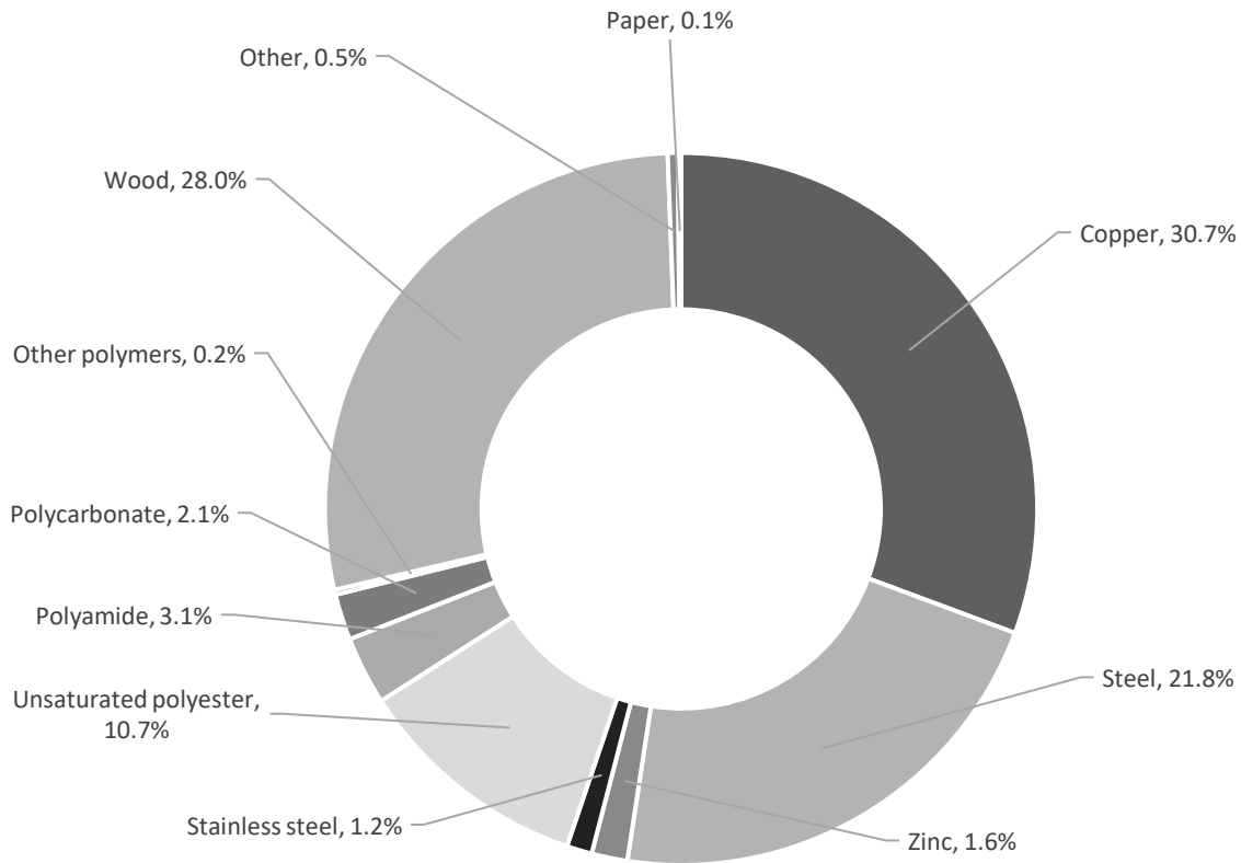
Figure 1: Composition of OTM4000E3M230C
