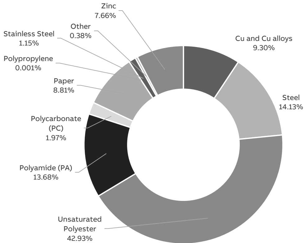
Figure1: Composition of OTDC250G-2P.
