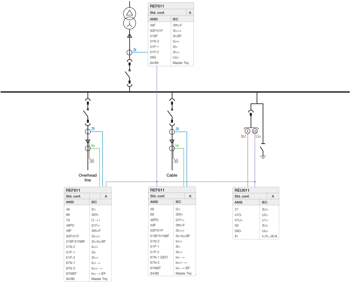
Figure 2. Busbar protection and supervision
