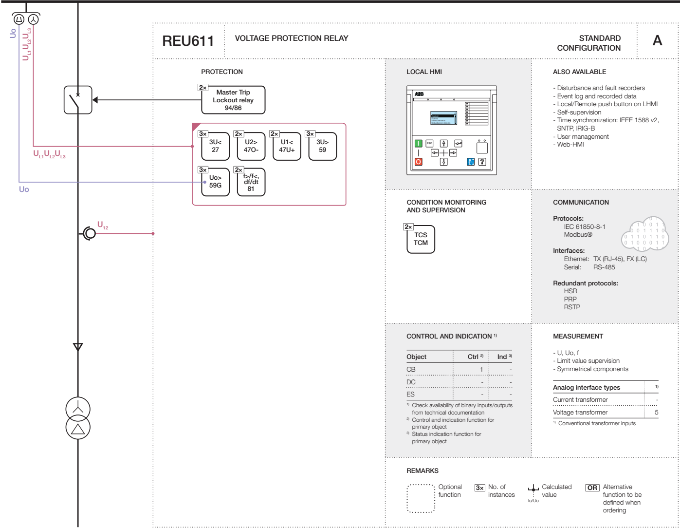
Figure 1. Functionality overview for configuration A
