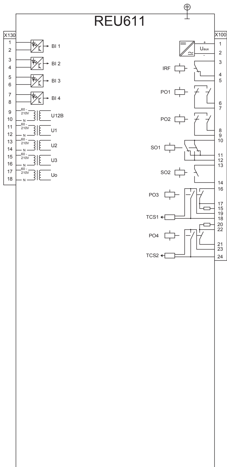
Figure 12. Terminal diagram of configuration A
