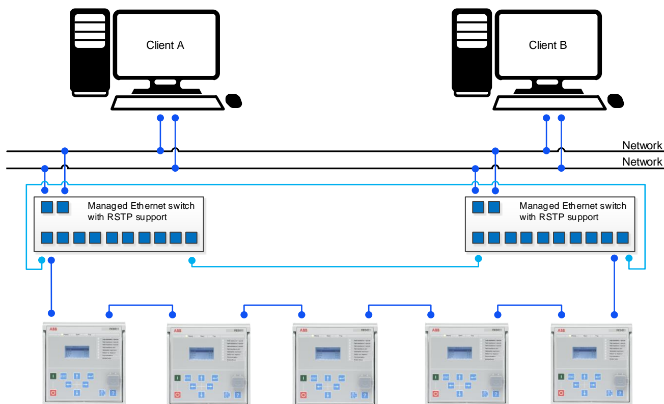
Figure 6. Self-healing Ethernet solution
