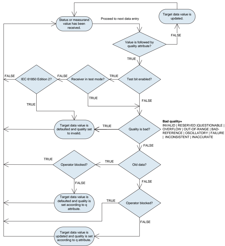
Figure 37: Receiving GOOSE data with quality in the merging units
