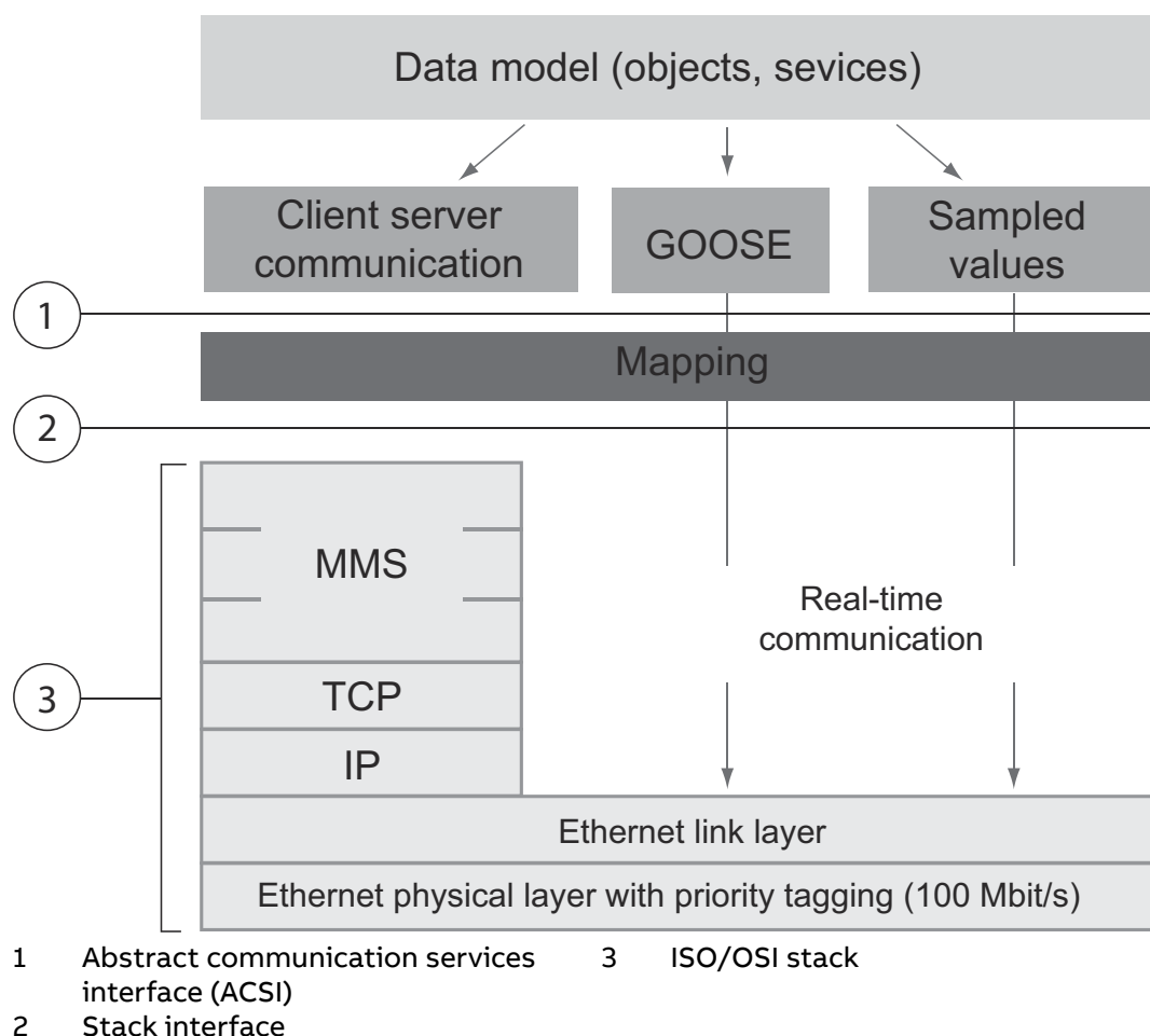
Figure 3: Communication stacks and mapping used in IEC 61850
