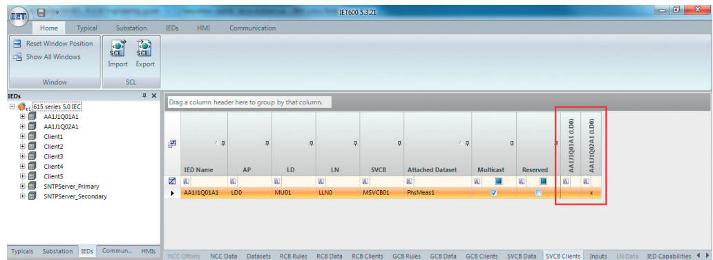
Figure 48: Connecting the SMV sender and receivers in IET600
