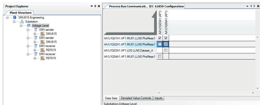
Figure 44: Configuring the SMV sender and receivers
