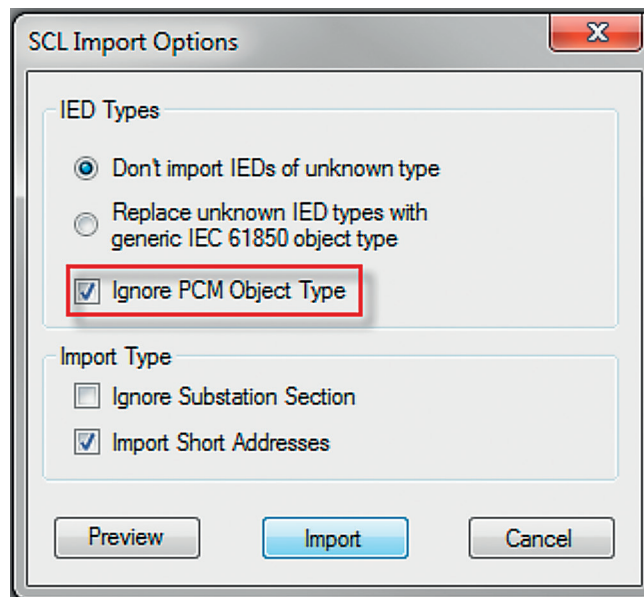
Figure 52: Defining SCL import options
