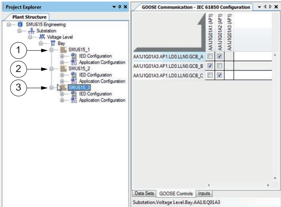
Figure 15: GCB client editor showing the senders and receivers
