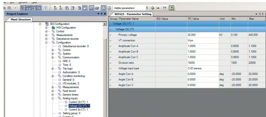
Figure 49: Amplitude and angle correction
