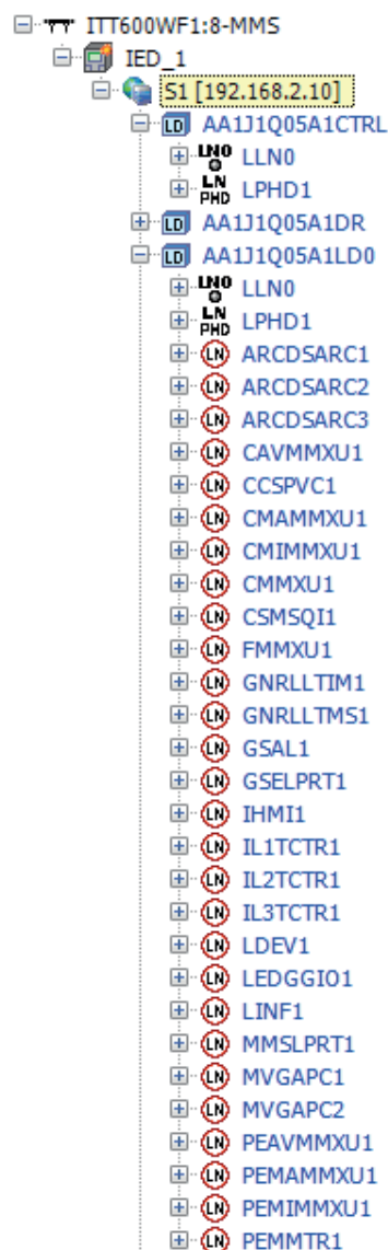
Figure 4: Example of an IEC 61850 data model of a merging unit
