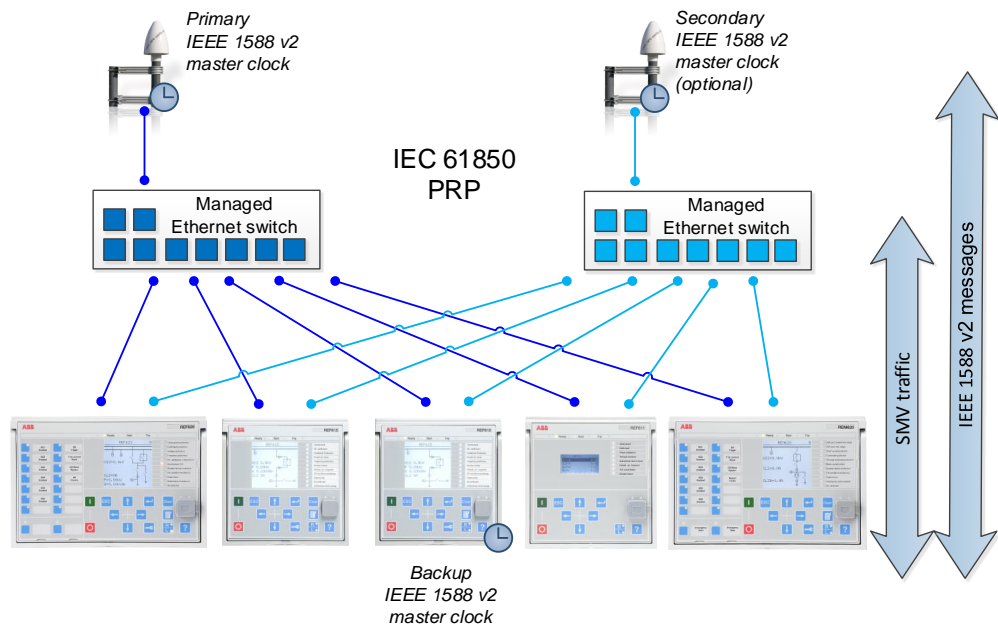
Figure 39: Recommended PRP reference topology with SMV and IEEE 1588 v2
