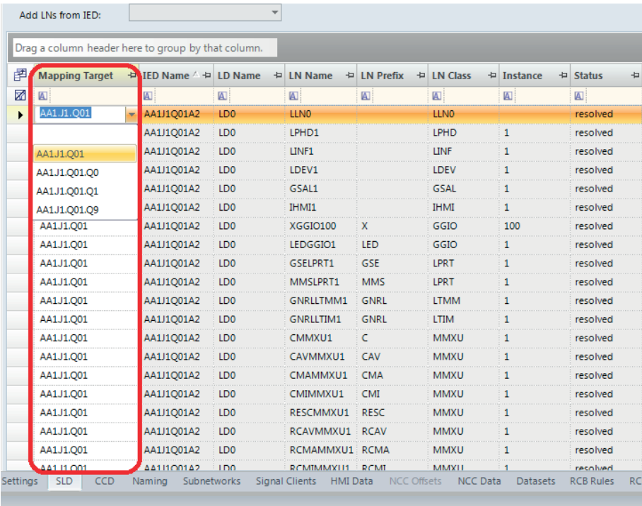
Figure 70: LN Mapping Editor
