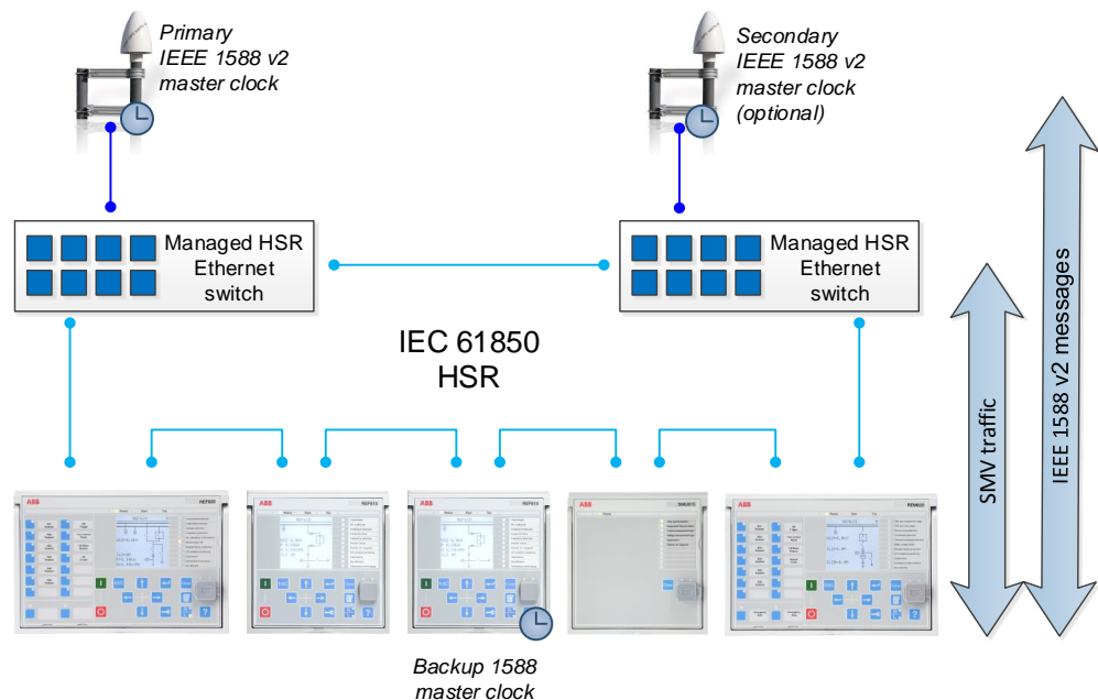
Figure 38: Recommended HSR reference topology with SMV and IEEE 1588 v2
