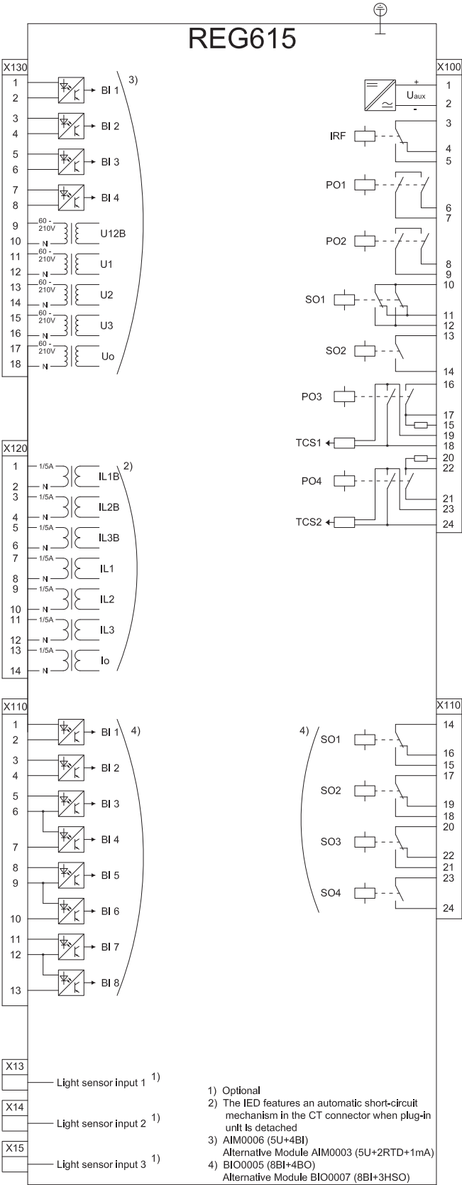
Figure 21. Terminal diagram of standard configuration D
