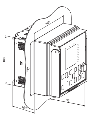
Figure 17. Semi-flush mounting
