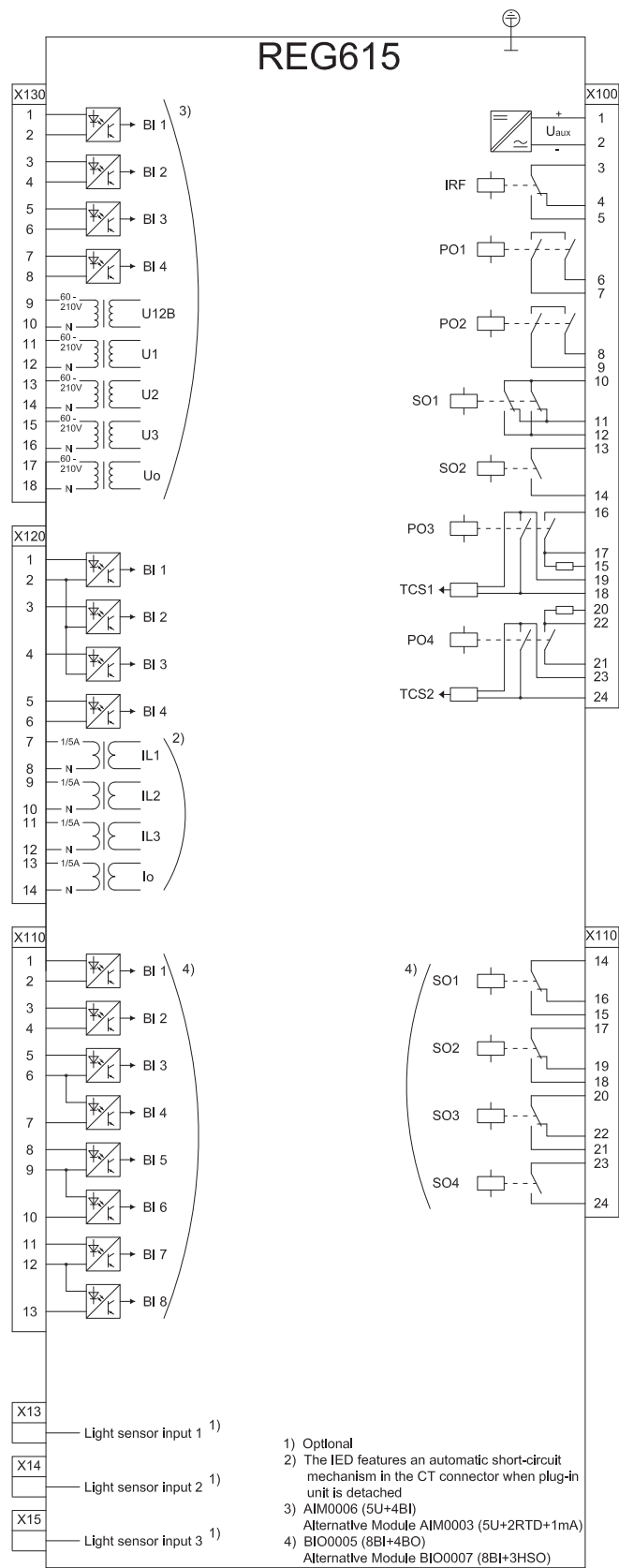
Figure 19. Terminal diagram of standard configuration A
