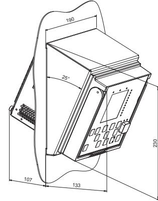
Figure 18. Semi-flush mounting in a 25° tilt
