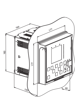
Figure 16. Flush mounting
