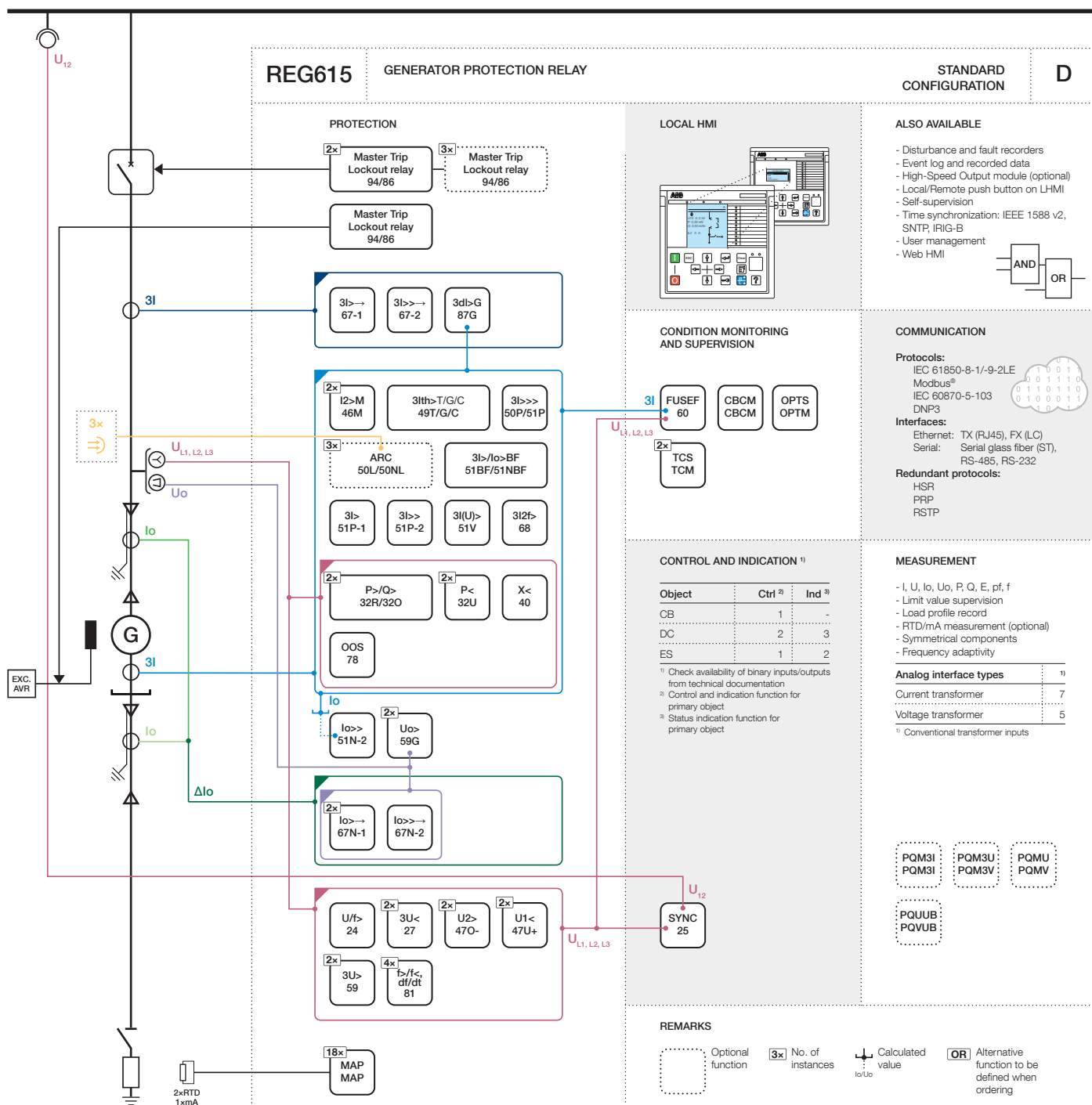
Figure 3. Functionality overview for standard configuration D
