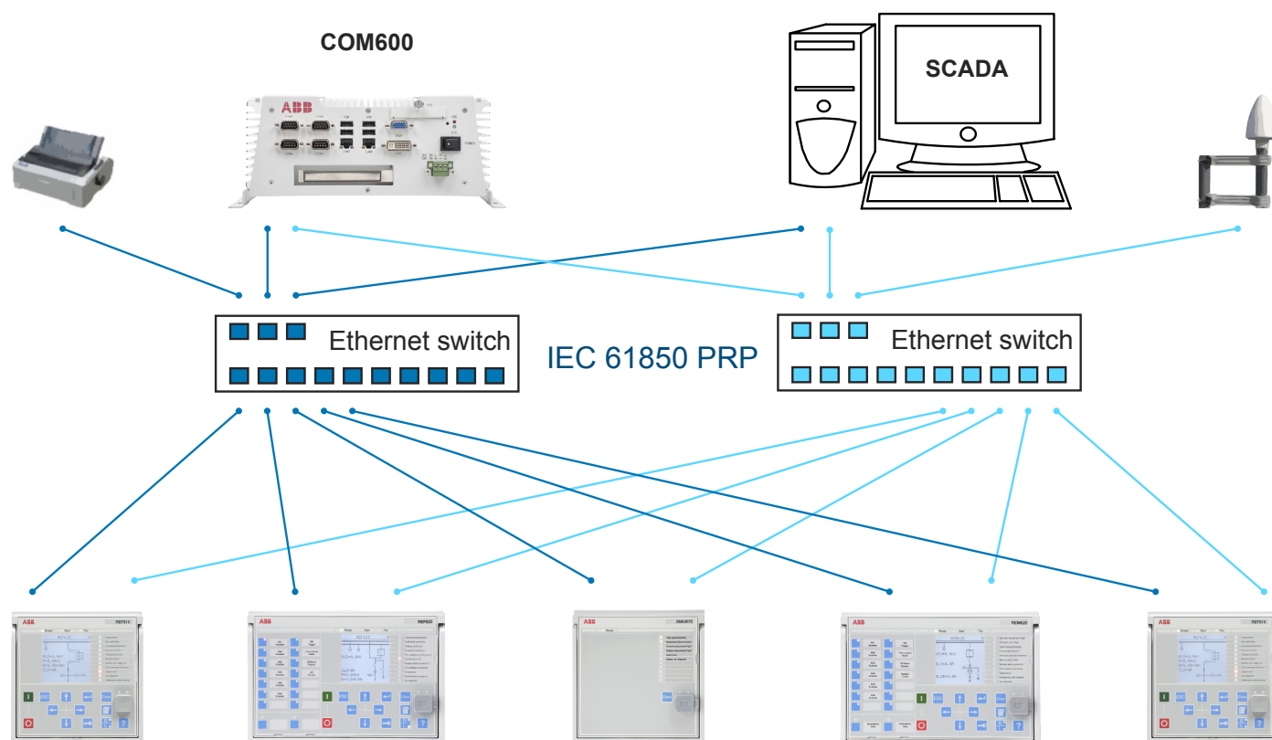
Figure 11. Parallel redundancy protocol (PRP) solution
