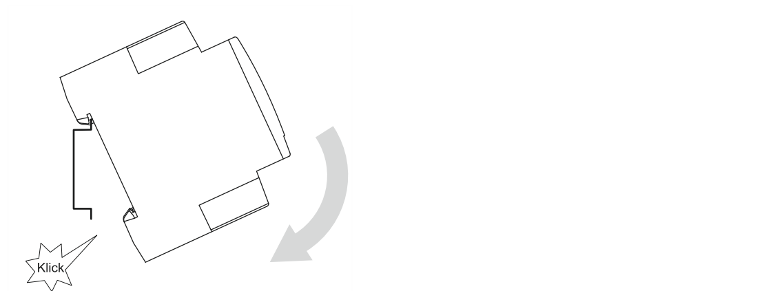
Fig. 3: Installation on mounting rails
