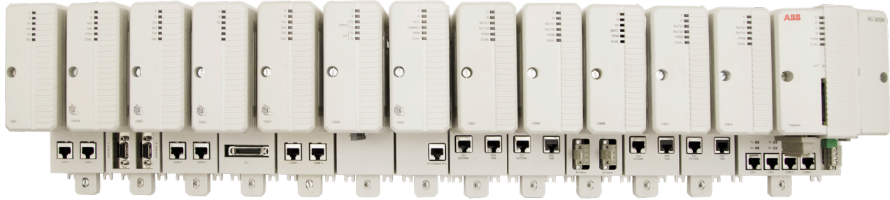
— AC 800M controller with 12 communication modules.
