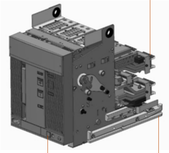
Emax 2 Closed Door mechanism
