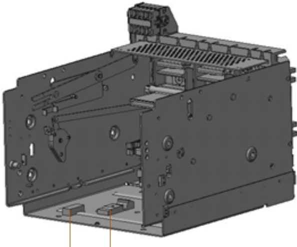
Megamax standard Fixed Part + matching connecting device for the Emax 2 racking in-out mechanism
