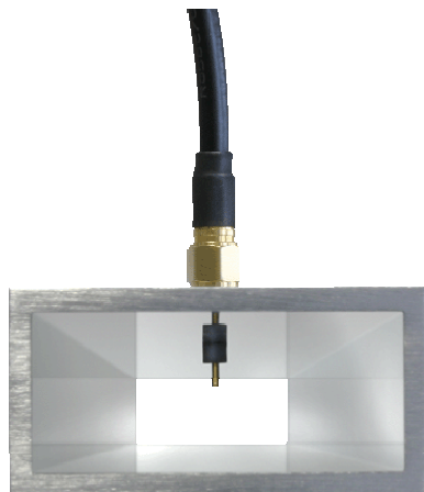
Figure 2. Typical hollow conductor with probe
