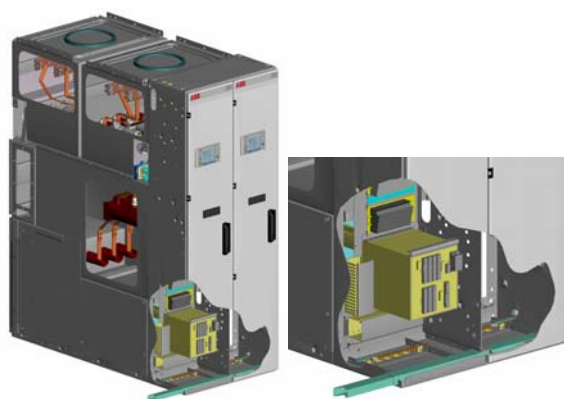
Figure 1. Gas-insulated MV switchgear type ZX2 with hollow conductor (l.), enlargement of the hollow conductor arrangement in the low voltage compartment (r.).
